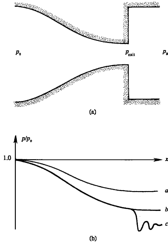
Figure 16.13 Pressure distribution along a convergent nozzle for different values of back pressure p_B : (a) diagram of nozzle; and (b) pressure distributions.
