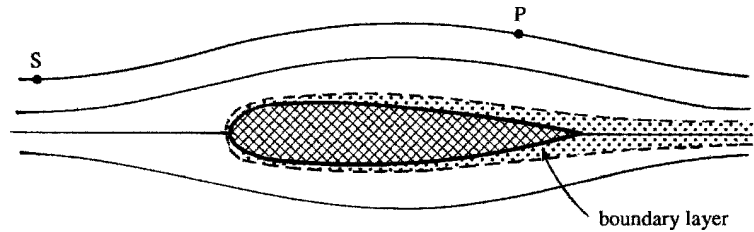
Figure 4.18 Flow over a solid object. Flow outside the boundary layer is irrotational.
