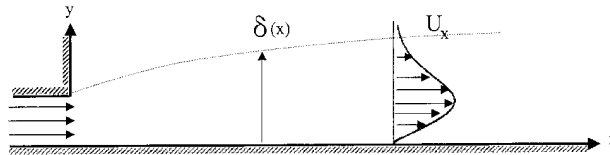
Figure 10.29 The planar wall jet.
