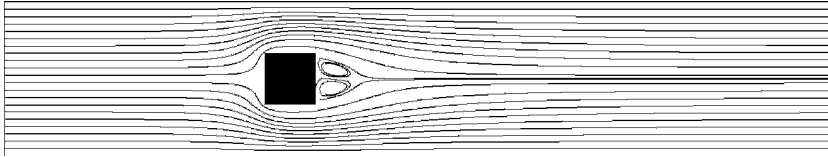
Figure 11.11 Streamlines for flow around a block at Re = 20 .
