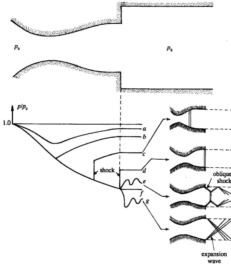
Figure 16.14 Pressure distribution along a convergent–divergent nozzle for different values of back pressure p_B . Flow patterns for cases c , d , e , and g are indicated schematically on the right. H. W. Liepmann and A. Roshko, Elements of Gas Dynamics , Wiley, New York 1957 and reprinted with the permission of Dr. Anatol Roshko.
