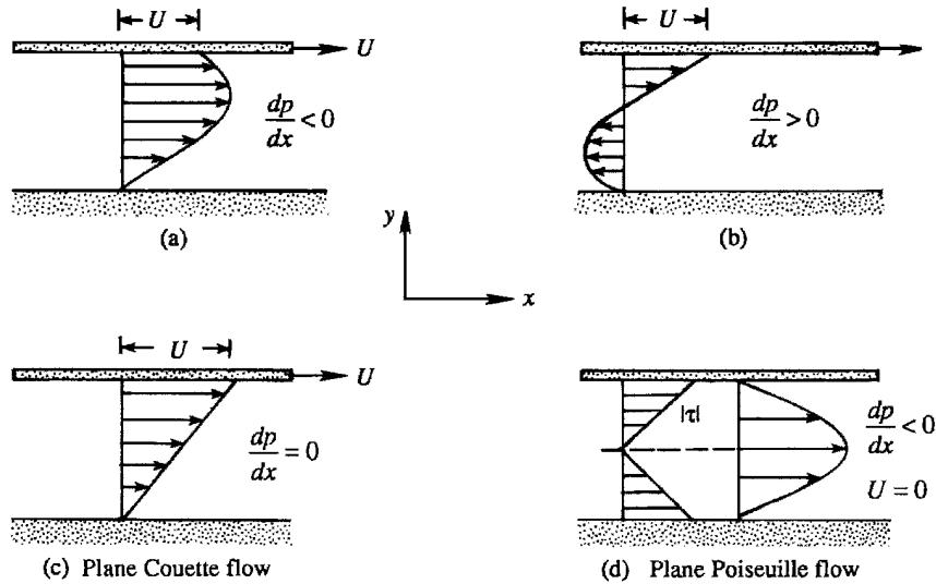
Figure 9.4 Various cases of parallel flow in a channel.
