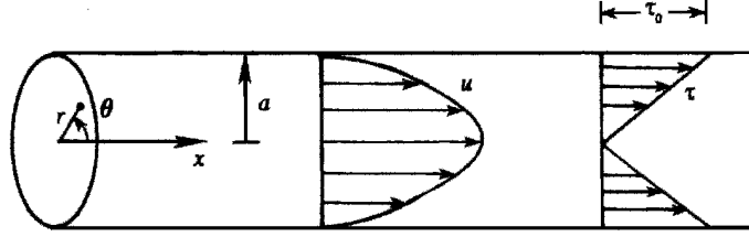
Figure 9.5 Laminar flow through a tube.
