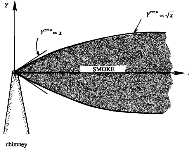
Figure 13.30 Average shape of a smoke plume in a wind blowing uniformly along the x -axis. G. I. Taylor, Proc. London Mathematical Society 20 : 196–211, 1921.
