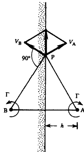
Figure 5.14 Line vortex A near a wall and its image B.
