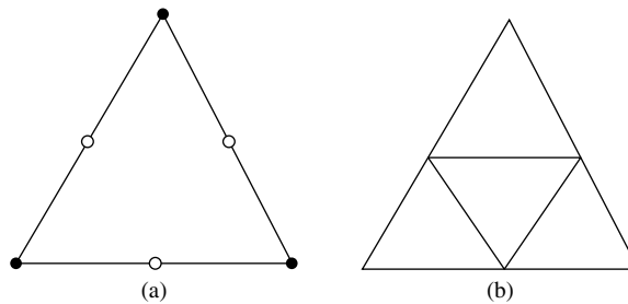
Figure 11.5 Mixed finite elements.
