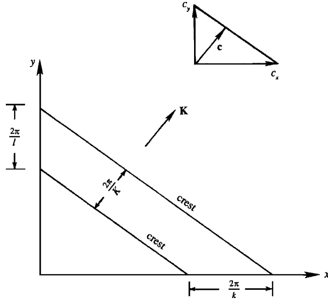
Figure 7.3 Wave propagating in the xy -plane. The inset shows how the components c_x and c_y are added to give the resultant \mathbf{c} .
