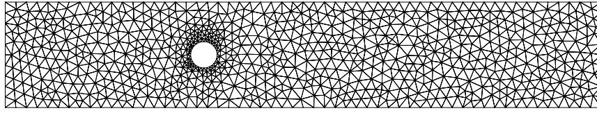
Figure 11.16 A finite element mesh around a cylinder.
