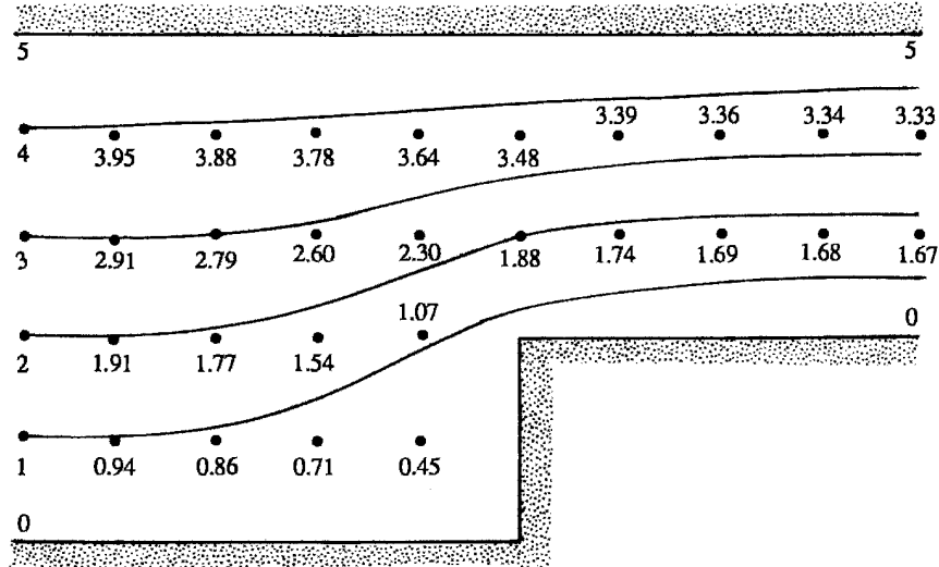
Figure 6.26 Numerical solution of Example 6.1.
