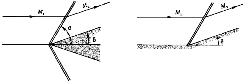
Figure 16.21 Oblique shocks in supersonic flow.
