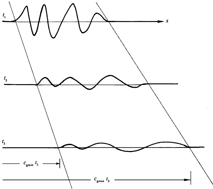
Figure 7.19 Surface profiles at three values of time due to a disturbance caused by dropping a stone into a pool.
