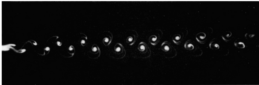
Figure 10.18 von Karman vortex street downstream of a circular cylinder at Re = 55 . Flow visualized by condensed milk. S. Taneda, Jour. Phys. Soc., Japan 20 : 1714–1721, 1965, and reprinted with the permission of The Physical Society of Japan and Dr. Sadatoshi Taneda.
