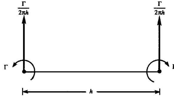
Figure 5.12 Interaction of line vortices of opposite spin, but of the same magnitude. Here \Gamma refers to the magnitude of circulation.
