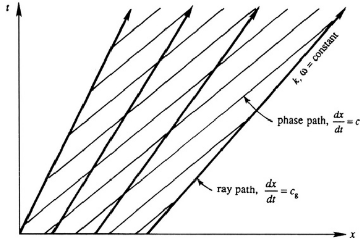
Figure 7.20 Propagation of a wave group in a homogeneous medium, represented on an xt -plot. Thin lines indicate paths taken by wave crests, and thick lines represent paths along which k and \omega are constant. M. J. Lighthill, Waves in Fluids , 1978 and reprinted with the permission of Cambridge University Press, London.
