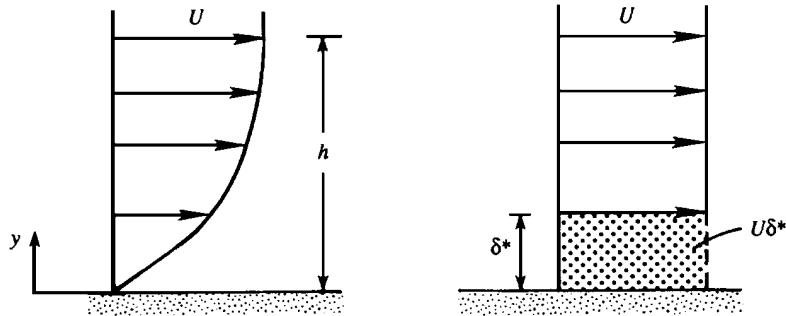
Figure 10.3 Displacement thickness.
