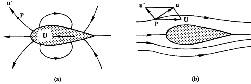
Figure 3.8 Flow past a ship with respect to two observers: (a) observer on river bank; (b) observer on ship.
