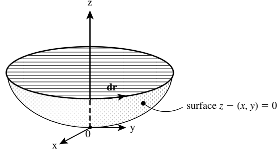
Figure 4.23 Geometry of equilibrium interface with surface tension.
