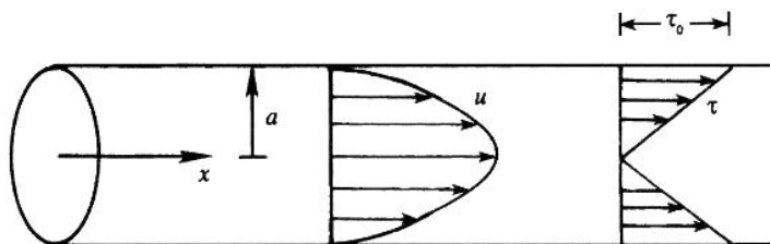
Figure 17.11 Poiseuille flow.
