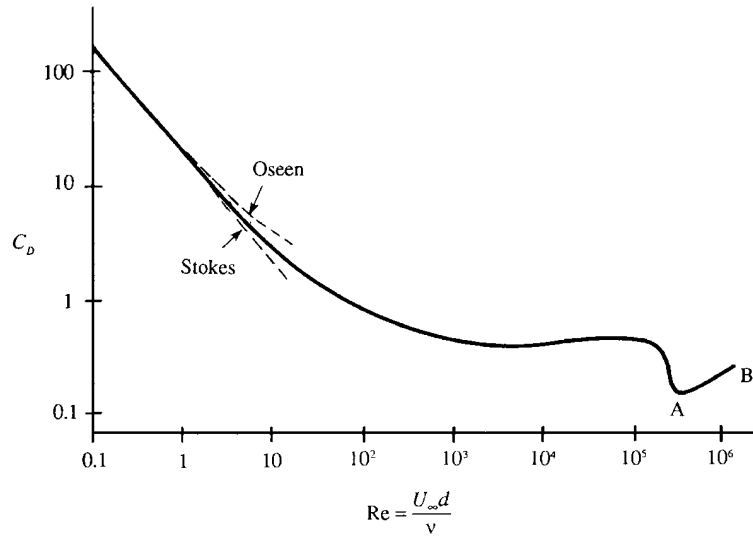
Figure 10.23 Measured drag coefficient of a smooth sphere. The Stokes solution is C_D = 24/\text{Re} , and the Oseen solution is C_D = (24/\text{Re})(1 + 3\text{Re}/16) ; these two solutions are discussed in Chapter 9, Sections 12 and 13. The increase of drag coefficient in the range AB has relevance in explaining why the flight paths of sports balls bend in the air.
