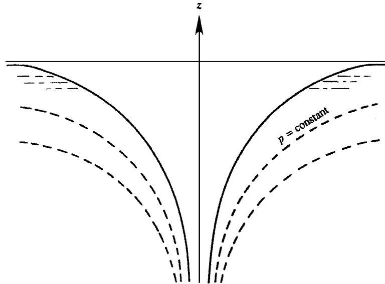
Figure 5.3 Irrotational vortex in a liquid.
