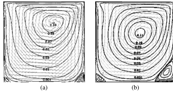
Figure 11.7 Comparisons of results from the explicit MacCormack scheme (light gray, velocity vector field) and those from Hou, et al. (1995) (dark solid streamlines) calculated using a Lattice Boltzmann Method. (a) Re = 100 , (b) at Re = 400 .
