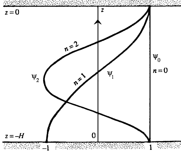
Figure 14.13 Vertical distribution of a few normal modes in a stratified medium of uniform buoyancy frequency.
