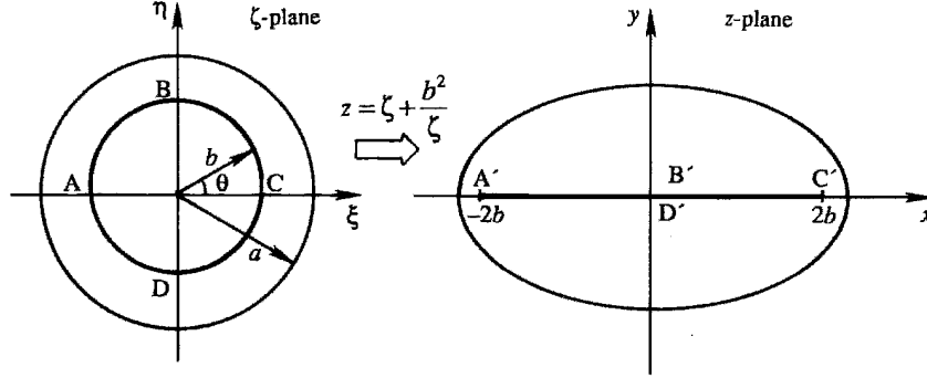
Figure 6.21 Transformation of a circle into an ellipse by means of the Zhukovsky transformation z = \zeta + b^2/\zeta .
