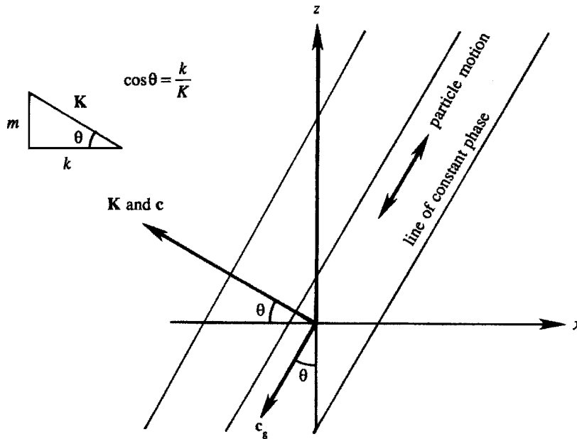
Figure 7.32 Basic parameters of internal waves. Note that \mathbf{c} and \mathbf{c}_g are at right angles and have opposite vertical components.
