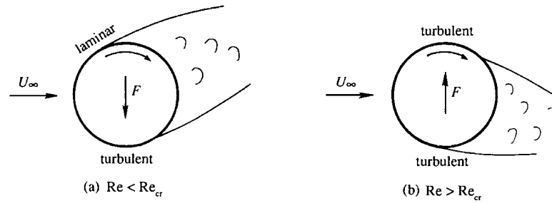
Figure 10.26 Bending of rotating spheres, in which F indicates the force exerted by the fluid: (a) negative Magnus effect; and (b) positive Magnus effect. A well-hit tennis ball is likely to display the positive Magnus effect.
