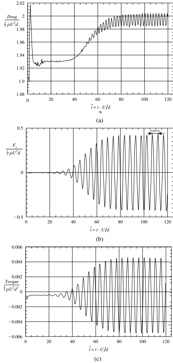
Figure 11.21 History of forces and torque acting on the cylinder at Re = 100 : (a) drag coefficient; (b) lift coefficient; and (c) coefficient for the torque.
