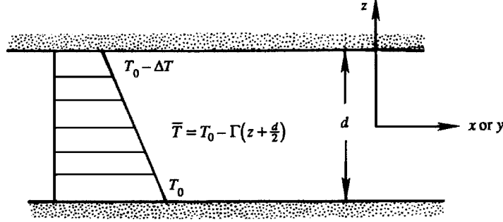
Figure 12.2 Definition sketch for the Bénard problem.
