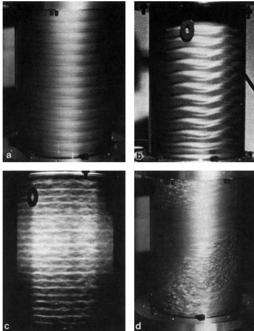
Figure 12.12 Instability of rotating Couette flow. Panels a, b, c, and d correspond to increasing Taylor number. D. Coles, Journal of Fluid Mechanics 21 : 385–425, 1965 and reprinted with the permission of Cambridge University Press.
