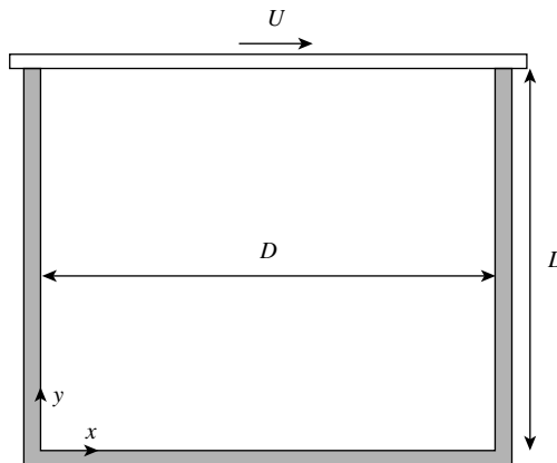
Figure 11.6 Driven cavity flow problem. The cavity is filled with a fluid with the top lid sliding at a constant velocity U .
