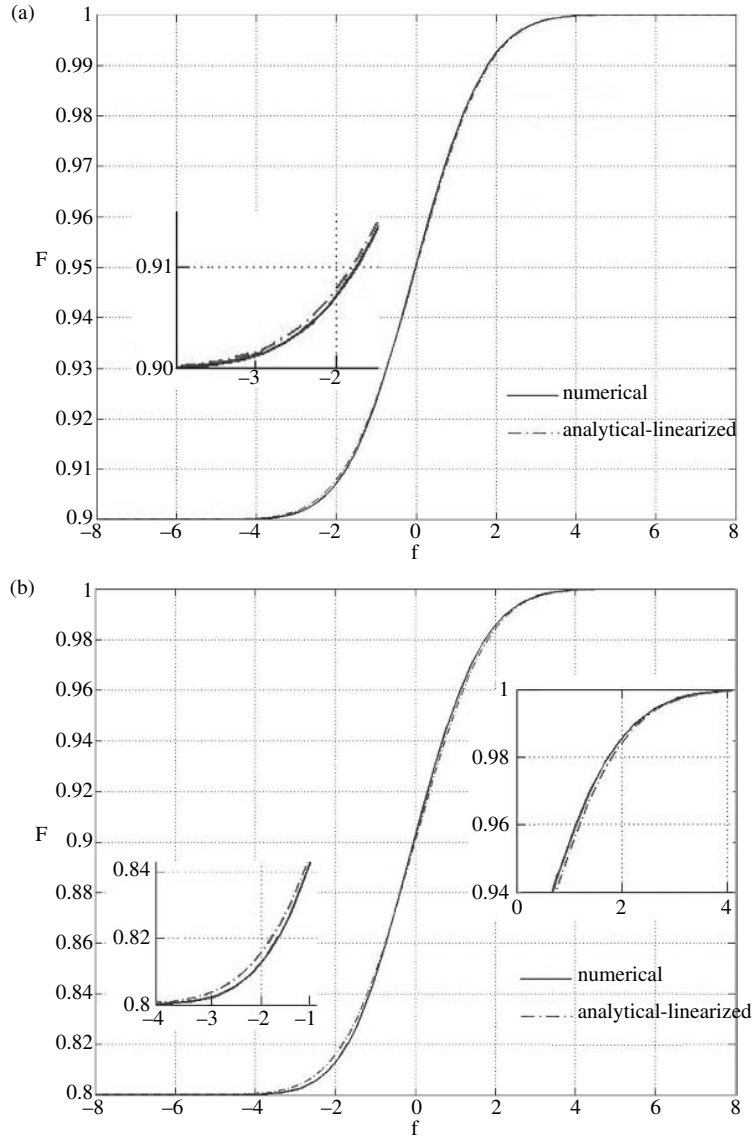
Figure 10.36 Solution for F(f) from equation (10.99) subject to boundary conditions (10.100) when (a) U_2/U_1 = 0.9 , and (b) U_2/U_1 = 0.8 . The “analytical—linearized” approximation is the asymptotic solution for (U_1 - U_2)/U_1 \ll 1 : F = 1 - [(U_1 - U_2)/(2U_1)]\text{erfc}(f/2) . Magnified insets show the difference between the two curves.
