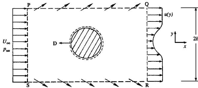
Figure 4.8 Momentum balance of flow over a body (Example 4.1).
