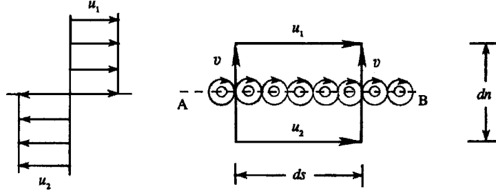
Figure 5.16 Vortex sheet.
