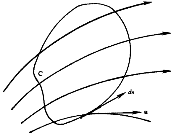
Figure 3.11 Circulation around contour C .
