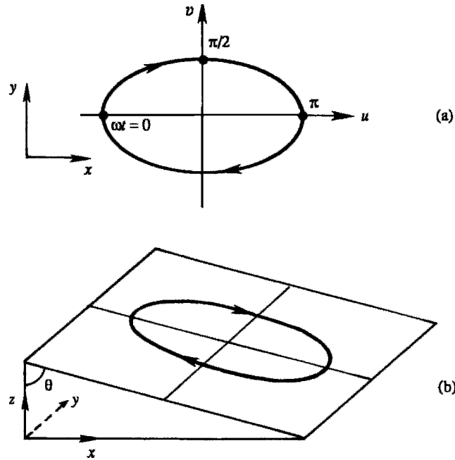
Figure 14.22 Particle orbit in an internal wave. The upper panel (a) shows projection on a horizontal plane; points corresponding to \omega t = 0, \pi/2 , and \pi are indicated. The lower panel (b) shows a three-dimensional view. Sense of rotation shown is valid for the northern hemisphere.
