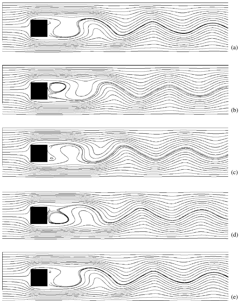
Figure 11.12 A sequence of flow fields around a block at Re = 100 during one period of vortex shedding. (a) t = 40.53 , (b) t = 41.50 , (c) t = 42.48 , (d) t = 43.45 , (e) t = 44.17 .
