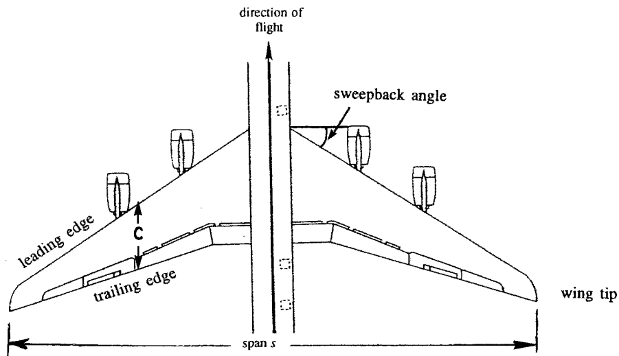
Figure 15.2 Wing planform geometry.
