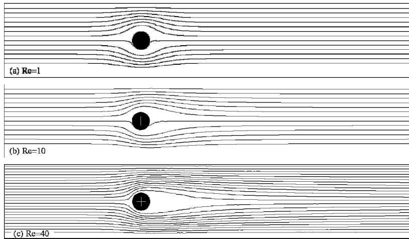
Figure 11.18 Streamlines for flow around a cylinder at three different Reynolds numbers.
