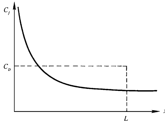
Figure 10.9 Friction coefficient and drag coefficient in a laminar boundary layer on a flat plate.
