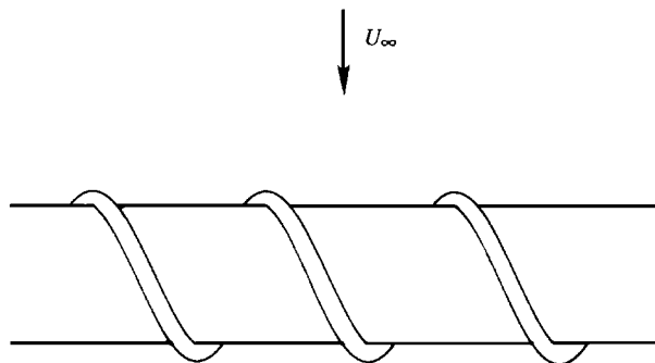
Figure 10.19 Spiral blades used for breaking up the spanwise coherence of vortex shedding from a cylindrical rod.
