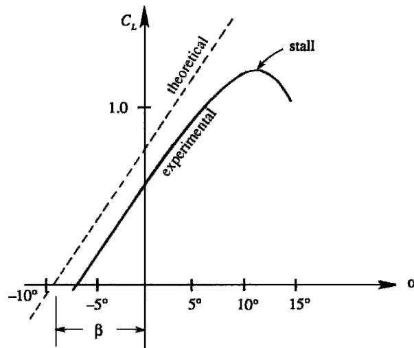
Figure 15.18 Comparison of theoretical and experimental lift coefficients for a cambered Zhukhovskiy airfoil.
