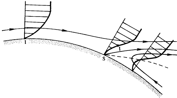
Figure 10.14 Streamlines and velocity profiles near a separation point S. Point of inflection is indicated by I. The dashed line represents u = 0 .
