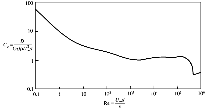
Figure 10.22 Measured drag coefficient of a circular cylinder. The sudden dip is due to the transition of the boundary layer to turbulence and the consequent downstream movement of the point of separation.
