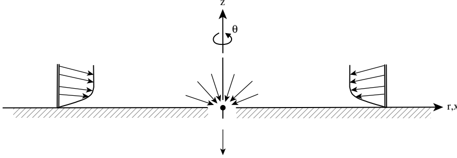
Figure 10.5 Axisymmetric flow into a sink at the center of an infinite plate.
