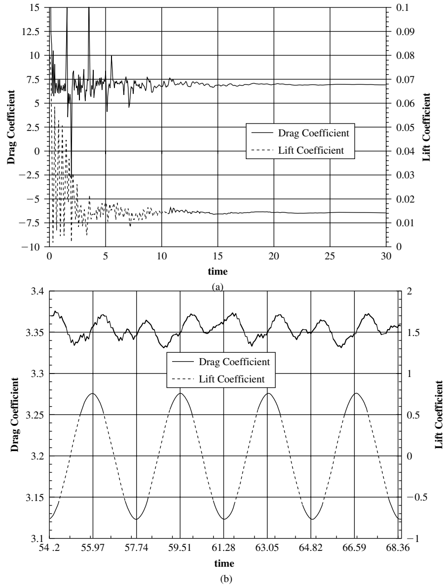
Figure 11.10 Drag and lift coefficients as functions of time for flow over a block. (a) Re = 20 , on a grid of 701 \times 61 , (b) Re = 100 , on a grid of 1401 \times 121 .
