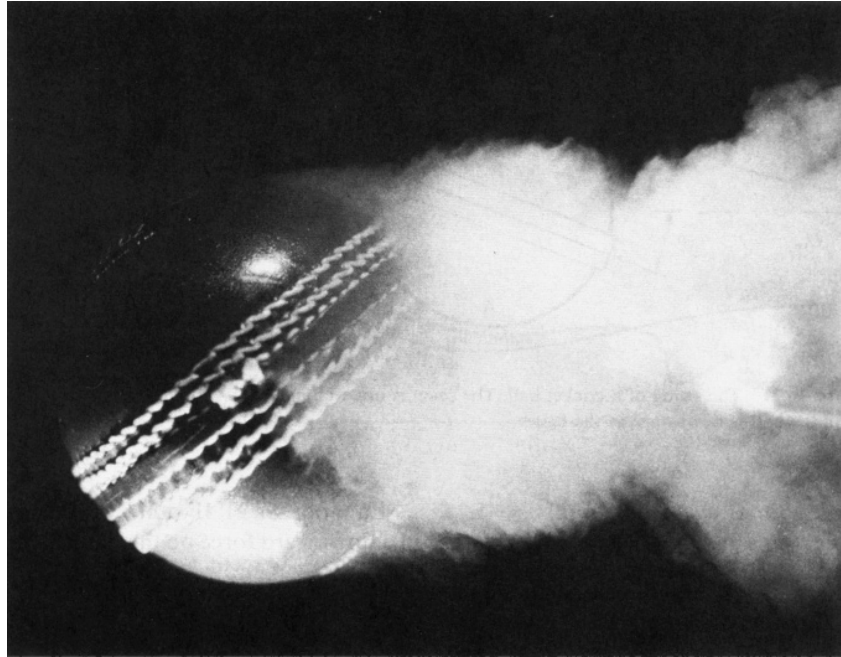
Figure 10.25 Smoke photograph of flow over a cricket ball. Flow is from left to right. Seam angle is 40^\circ , flow speed is 17 m/s, Re = 0.85 \times 10^5 . R. Mehta, Ann. Rev Fluid Mech. 17 : 151–189, 1985. Photograph reproduced with permission from the Annual Review of Fluid Mechanics , Vol. 17 © 1985 Annual Reviews www.AnnualReviews.org .
