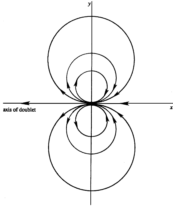
Figure 6.8 Plane doublet.
