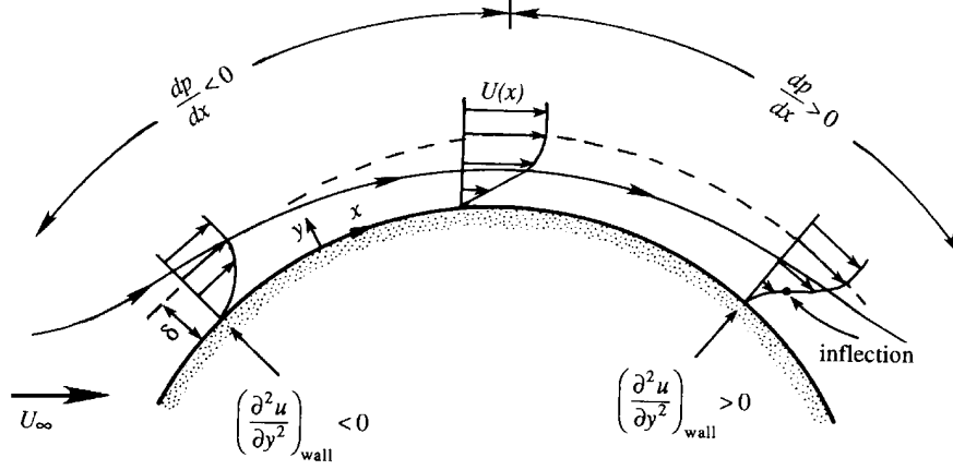
Figure 10.13 Velocity profiles across boundary layers with favorable and adverse pressure gradients.
