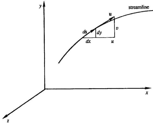
Figure 3.5 Streamline.
