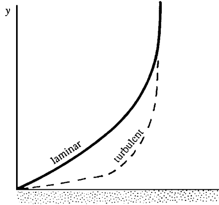
Figure 10.15 Comparison of laminar and turbulent velocity profiles in a boundary layer.
