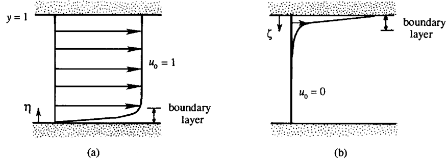
Figure 10.34 Couette flow with strong suction, showing two possible locations of the boundary layer. The one shown in (a) is the correct one.
