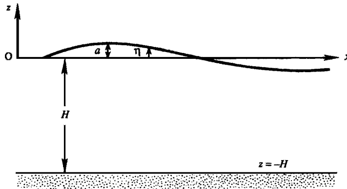
Figure 7.4 Wave nomenclature.
