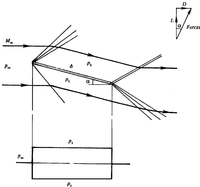
Figure 16.25 Inclined flat plate in a supersonic stream. The upper panel shows the flow pattern and the lower panel shows the pressure distribution.
