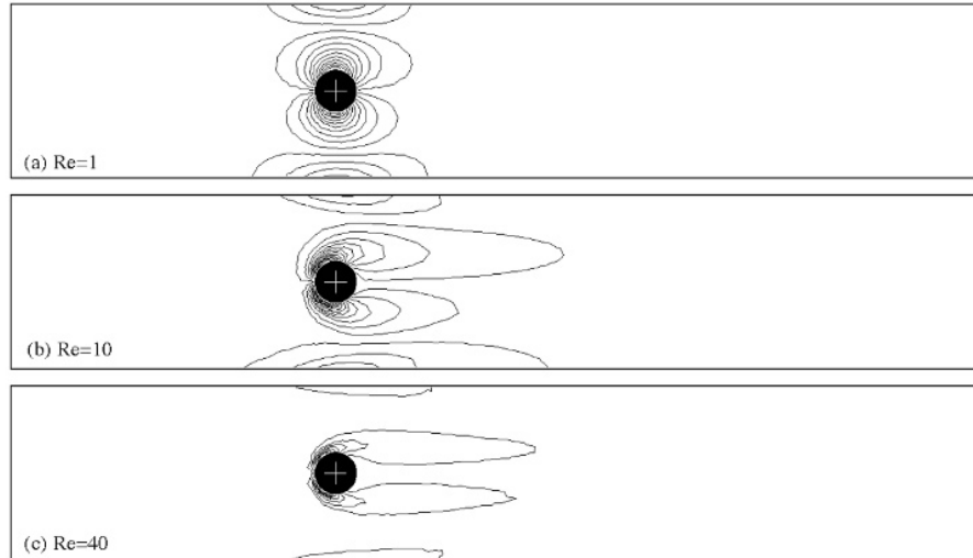
Figure 11.19 Vorticity lines for flow around a cylinder at three different Reynolds numbers.
