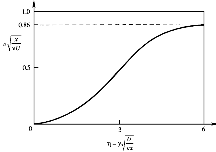
Figure 10.8 Transverse velocity component in a laminar boundary layer on a flat plate.
