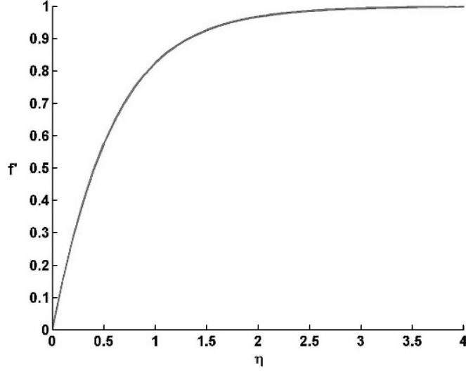
Figure 10.6 Dimensionless velocity profile for flow illustrated in Figure 10.5.
