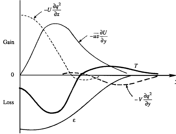
Figure 13.16 Sketch of observed kinetic energy budget in a turbulent jet. Turbulent transport is indicated by T .
