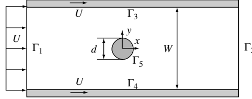
Figure 11.15 Flow geometry of flow around a cylinder in a channel.
