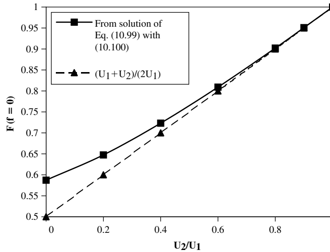
Figure 10.37 Comparison of streamwise velocity at dividing streamline ( f = 0 ) with average velocity (dashed line).
