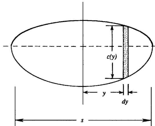
Figure 15.25 Wing of elliptic planform.
