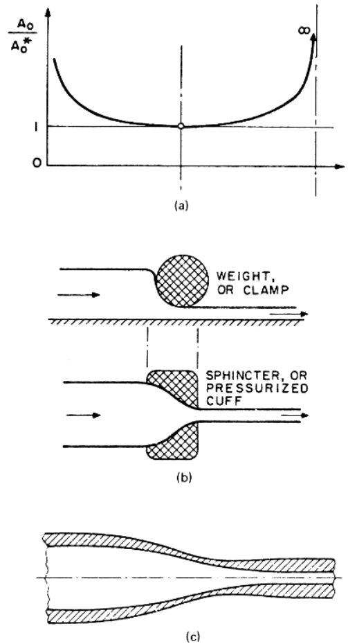
Figure 17.20 Smooth transition through the critical condition. (Reproduced with permission from the American Society of Mechanical Engineers, NY.).
