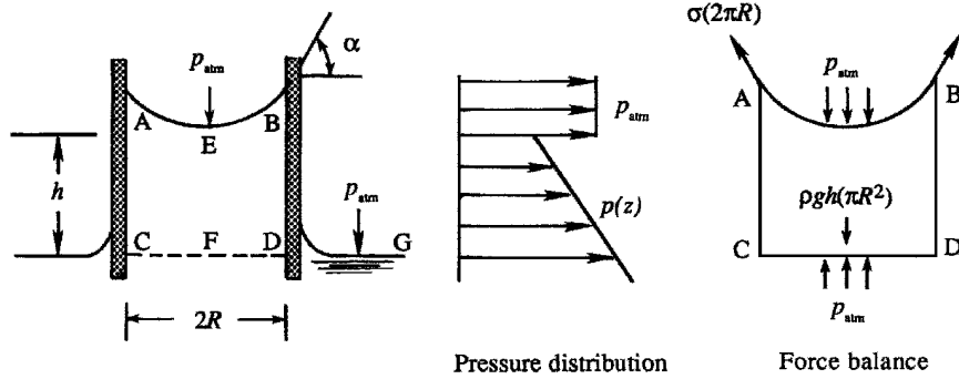
Figure 1.7 Rise of a liquid in a narrow tube (Example 1.1).
