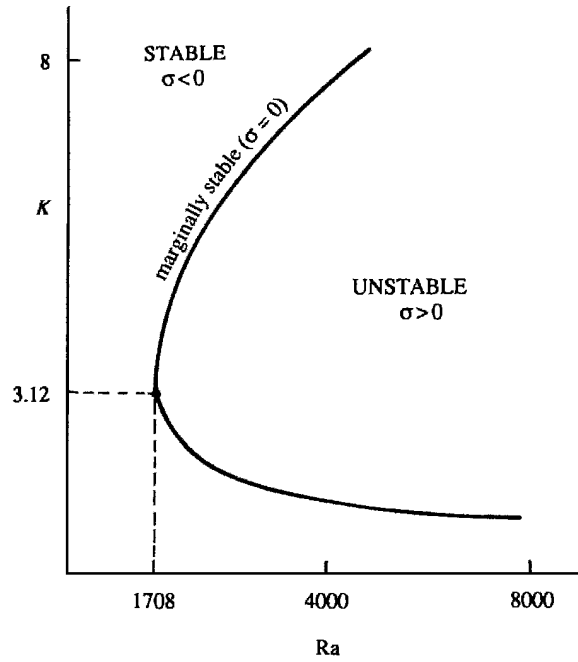
Figure 12.4 Stable and unstable regions for Bénard convection.
