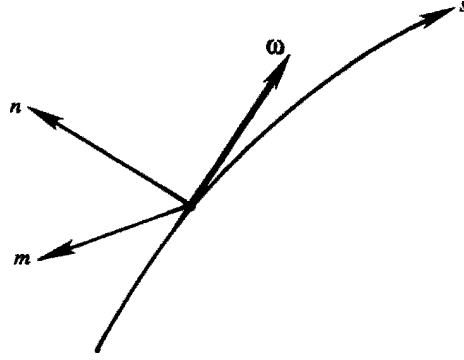
Figure 5.9 Coordinate system aligned with vorticity vector.
