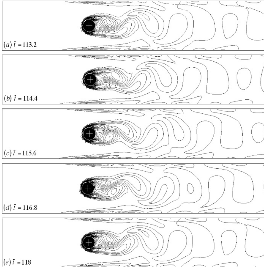
Figure 11.20 Vorticity lines for flow around a cylinder at Reynolds number Re = 100 . \bar{t} = tU/d is the dimensionless time.
