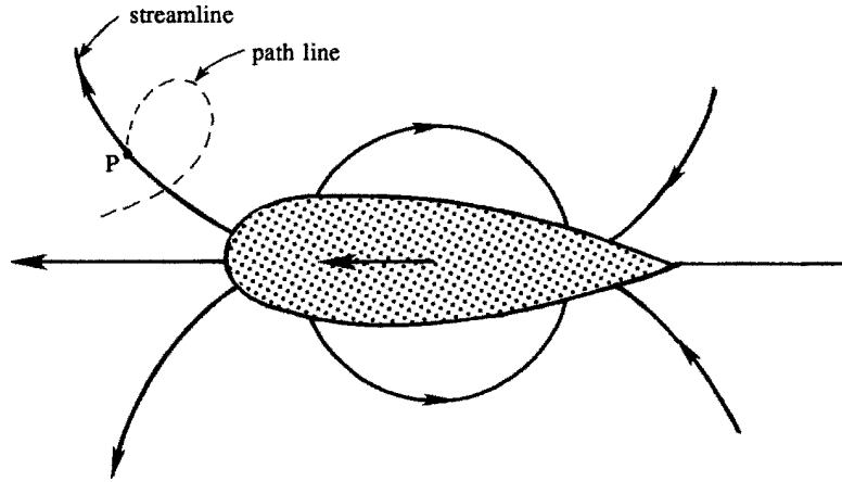
Figure 3.7 Several streamlines and a path line due to a moving body.
