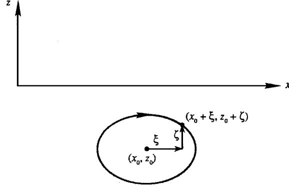
Figure 7.5 Orbit of a fluid particle whose mean position is (x_0, z_0) .
