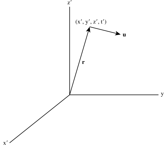
Figure 3.3 Field—Eulerian description. Independent variables: (x', y', z', t') ; dependent variables: \mathbf{u}(\mathbf{r}', t') , \rho(\mathbf{r}', t) , and so on.
