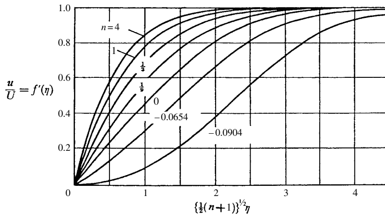
Figure 10.10 Velocity distribution in the boundary layer for external stream U_e = ax^n . G. K Batchelor, An Introduction to Fluid Dynamics , 1st ed. (1967), reprinted with the permission of Cambridge University Press.
