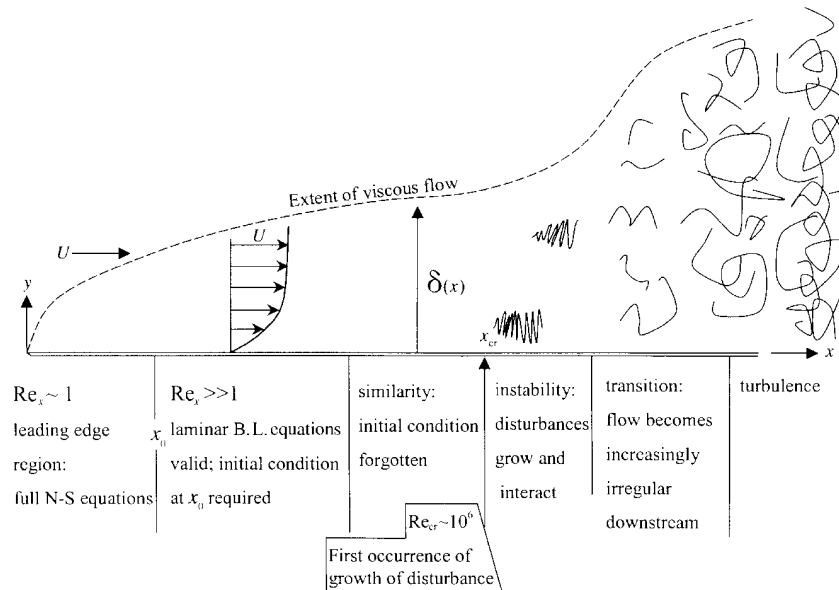
Figure 10.11 Schematic depiction of flow over a semiinfinite flat plate.
