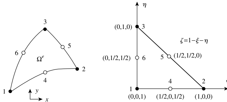
Figure 11.17 A quadratic triangular finite element mapping into the standard element.
