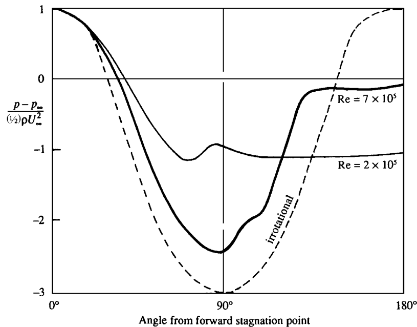
Figure 10.21 Surface pressure distribution around a circular cylinder at subcritical and supercritical Reynolds numbers. Note that the pressure is nearly constant within the wake and that the wake is narrower for flow at supercritical Re .
