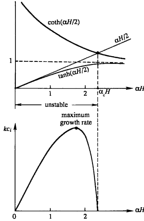
Figure 14.31 Baroclinic instability. The upper panel shows behavior of the functions in equation (14.141), and the lower panel shows growth rates of unstable waves.
