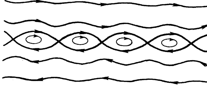
Figure 12.22 The Kelvin cat's eye pattern near a critical layer, showing streamlines as seen by an observer moving with the wave.
