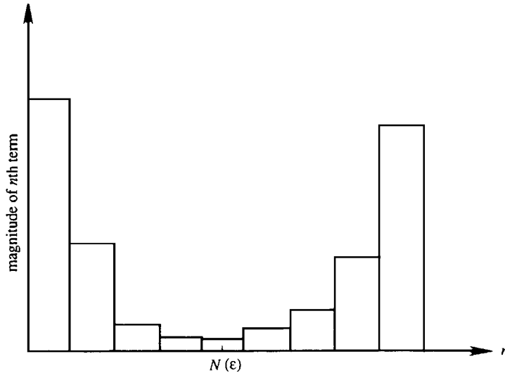
Figure 10.32 Terms in a divergent asymptotic series, in which N(\varepsilon) indicates the optimum number of terms at which the series should be truncated. M. Van Dyke, Perturbation Methods in Fluid Mechanics , 1975 and reprinted with the permission of Prof. Milton Van Dyke for The Parabolic Press.
