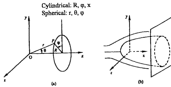
Figure 6.27 (a) Cylindrical and spherical coordinates; (b) axisymmetric flow. In Fig. 6.27, the coordinate axes are not aligned according to the conventional definitions. Specifically in (a), the polar axis from which \theta is measured is usually taken to be the z -axis and \varphi is measured from the x -axis. In (b), the axis of symmetry is usually taken to be the z -axis and the angle \theta or \varphi is measured from the x -axis.
