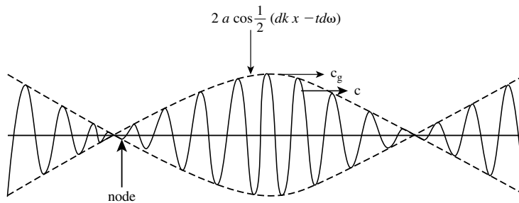
Figure 7.16 Linear combination of two sinusoids, forming repeated wave groups.
