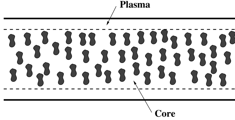
Figure 17.12 Fahraeus-Lindqvist effect.
