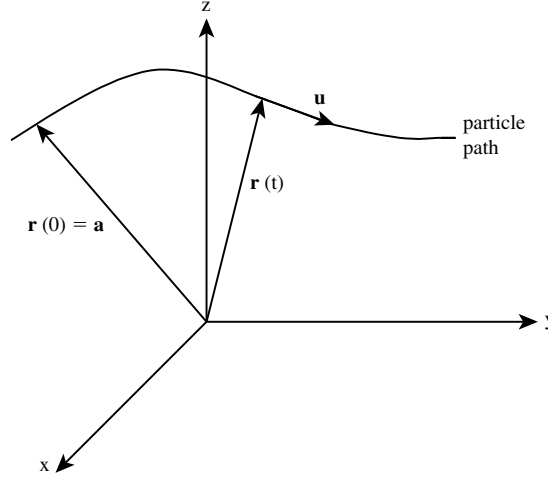
Figure 3.2 Particle—Lagrangian description. Independent variables: (\mathbf{a}, t) ; dependent variables: \mathbf{r}(\mathbf{a}, t) , \mathbf{u} = (\partial \mathbf{r} / \partial t)_{\mathbf{a}} , \rho = \rho(\mathbf{a}, t) , and so on.
