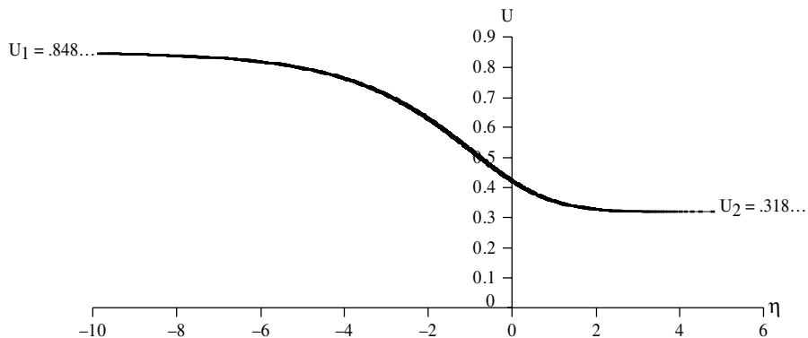
Figure 16.12 Shock structure velocity profile for the case U_1 = 0.848485 , U_2 = 0.31818 , corresponding to M_1 = 2.187 .
