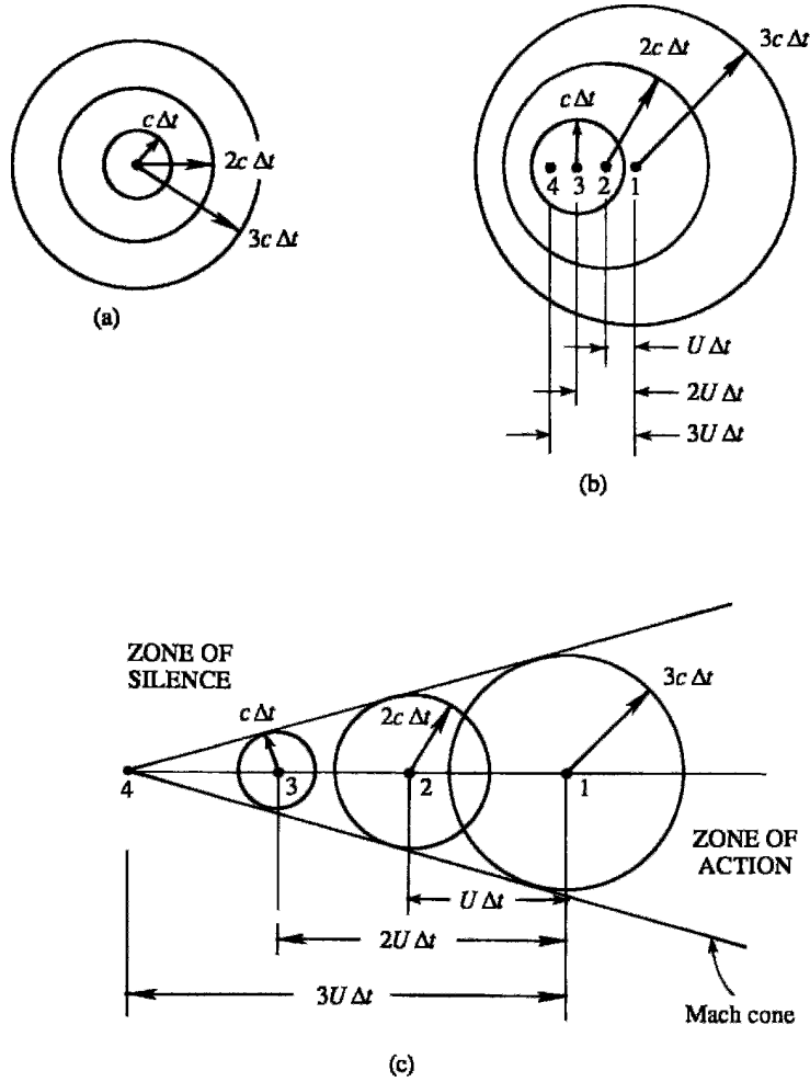
Figure 16.18 Wavefronts emitted by a point source in a still fluid when the source speed U is: (a) U = 0 ; (b) U < c ; and (c) U > c .
