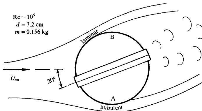
Figure 10.24 The swing of a cricket ball. The seam is oriented in such a way that the lateral force on the ball is downward in the figure.
