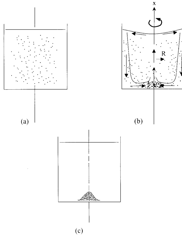
Figure 10.31 Secondary flow in a tea cup: (a) tea leaves randomly dispersed—initial state; (b) stirred vigorously—transient motion; and (c) final state.
