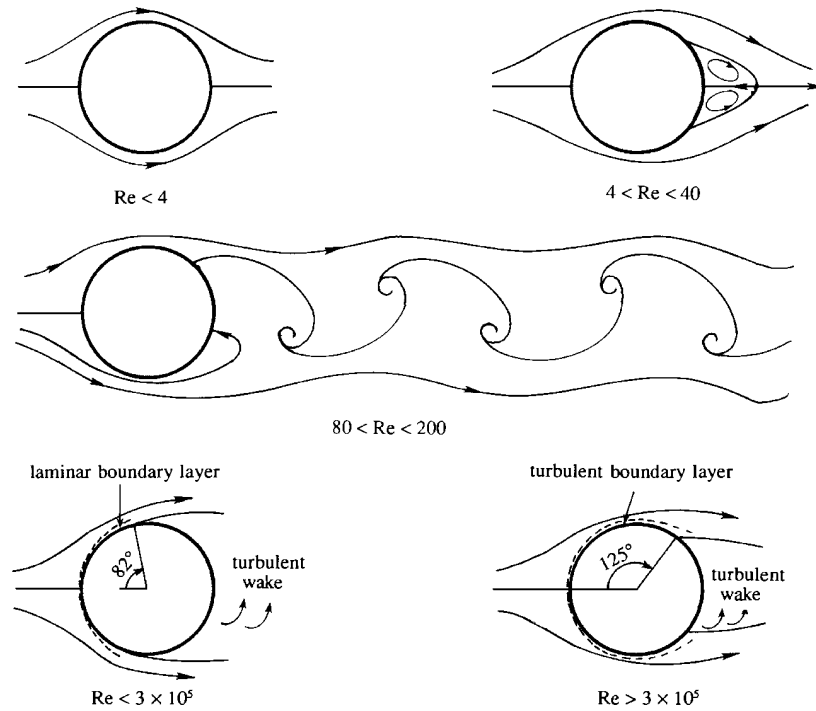
Figure 10.17 Some regimes of flow over a circular cylinder.
