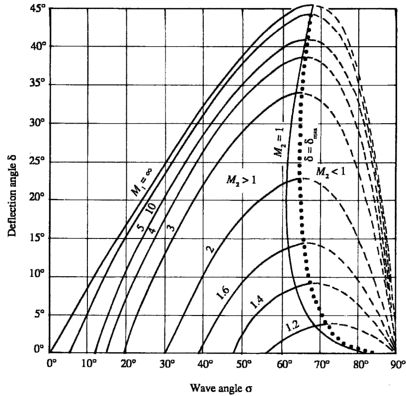
Figure 16.20 Plot of oblique shock solution. The strong shock branch is indicated by dashed lines, and the heavy dotted line indicates the maximum deflection angle \delta_{\max} . (From NACA Report 1135.)
