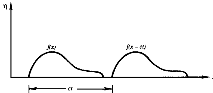
Figure 7.1 Profiles of f(x - ct) at two times.
