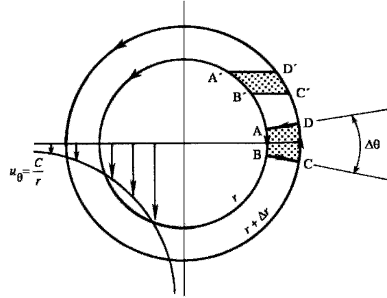
Figure 3.16 Irrotational vortex. Vorticity of a fluid element is infinite at the origin and zero everywhere else.
