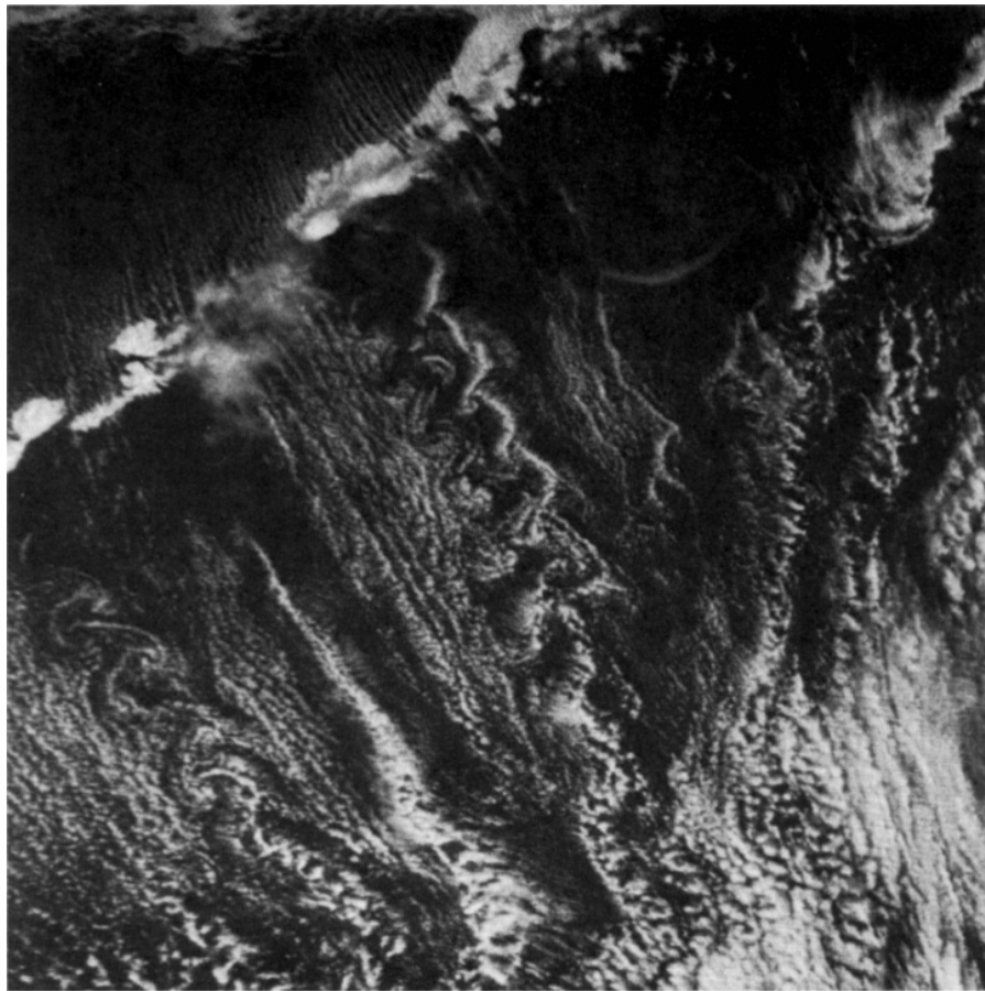
Figure 10.20 A von Karman vortex street downstream of mountain peaks in a strongly stratified atmosphere. There are several mountain peaks along the linear, light-colored feature running diagonally in the upper left-hand corner of the photograph. North is upward, and the wind is blowing toward the southeast. R. E. Thomson and J. F. R. Gower, Monthly Weather Review 105 : 873–884, 1977, and reprinted with the permission of the American Meteorological Society.
