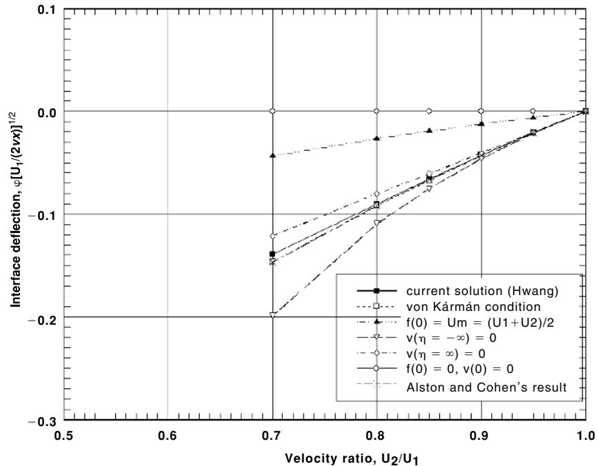
Figure 10.38 Asymptotic downstream dividing streamline deflection as a function of velocity ratio.
