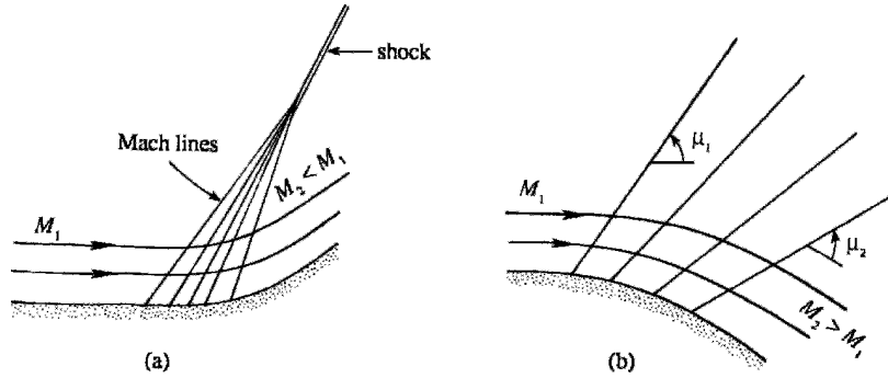
Figure 16.23 Gradual compression and expansion in supersonic flow: (a) gradual compression, resulting in shock formation; and (b) gradual expansion.
