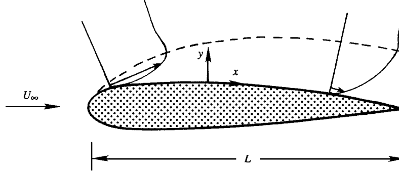
Figure 10.2 Velocity profiles at two positions within the boundary layer. The velocity arrows are drawn at the same distance y from the surface, showing that the variation of u with x is of the order of the free stream velocity U_\infty . The boundary layer thickness is greatly exaggerated.
