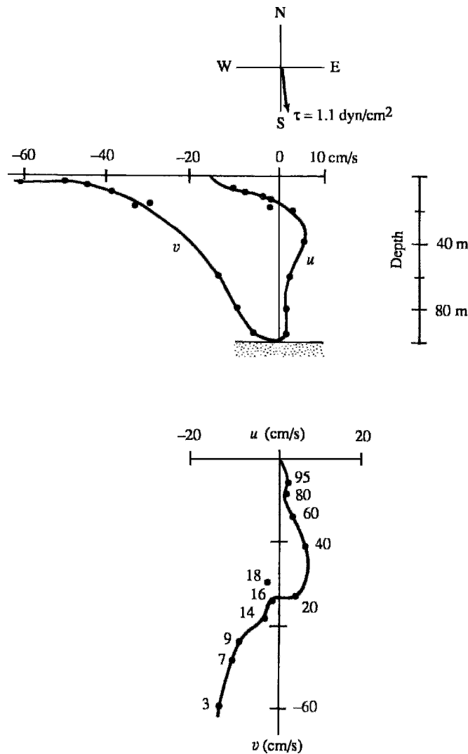
Figure 14.8 An observed velocity distribution near the coast of Oregon. Velocity is averaged over 7 days. Wind stress had a magnitude of 1.1 \text{ dyn/cm}^2 and was directed nearly southward, as indicated at the top of the figure. The upper panel shows vertical distributions of u and v , and the lower panel shows the hodograph in which depths are indicated in meters. The hodograph is similar to that of a surface Ekman layer (of depth 16 m) lying over the bottom Ekman layer (extending from a depth of 16 m to the ocean bottom). P. Kundu, in Bottom Turbulence , J. C. J. Nihoul, ed., Elsevier, 1977 and reprinted with the permission of Jacques C. J. Nihoul.
