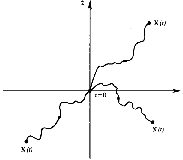
Figure 13.27 Three experimental outcomes of \mathbf{X}(t) , the current positions of particles from the origin at time t = 0 .
