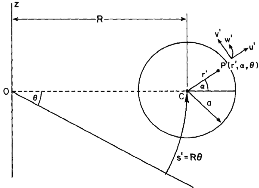
Figure 17.18 Toroidal coordinate system.
