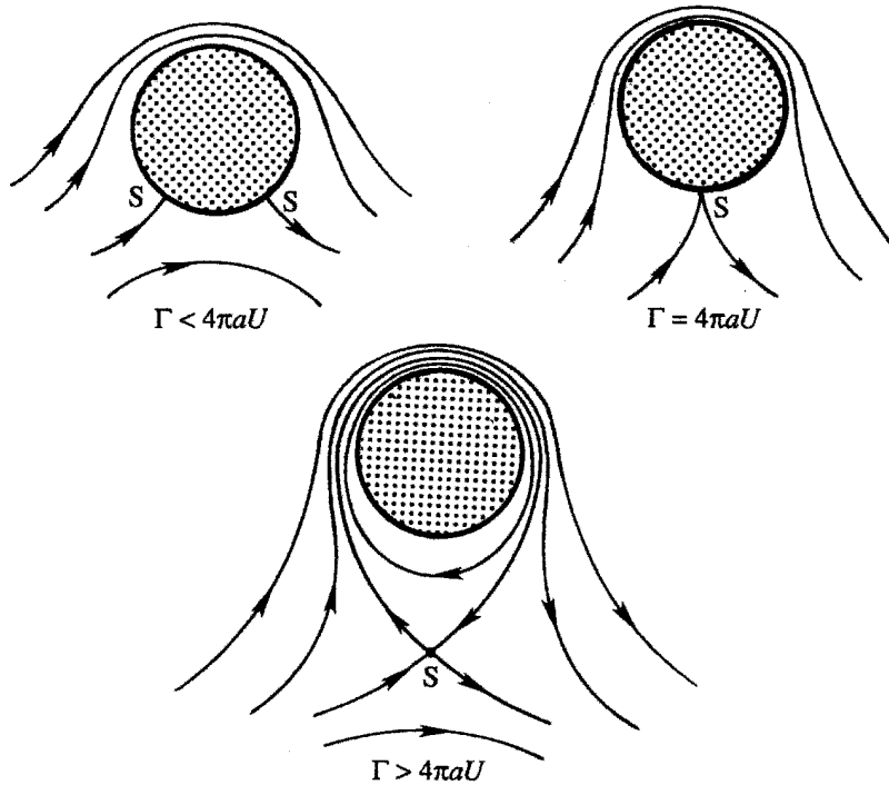
Figure 6.14 Irrotational flow past a circular cylinder for different values of circulation. Point S represents the stagnation point.
