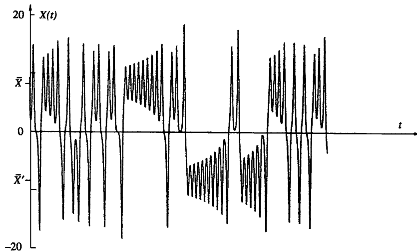
Figure 12.29 Variation of X(t) in the Lorenz model. Note that the solution oscillates erratically around the two steady values \bar{X} and \bar{X}' . P. Bergé, Y. Pomeau, and C. Vidal, Order Within Chaos , 1984 and reprinting permitted by Heinemann Educational, a division of Reed Educational & Professional Publishing Ltd.
