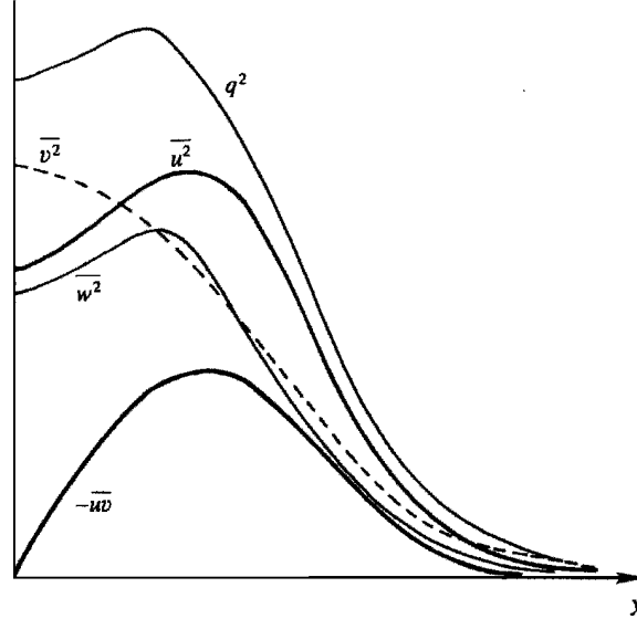
Figure 13.15 Sketch of observed variation of turbulent intensity and Reynolds stress across a jet.
