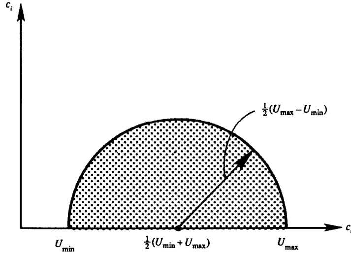
Figure 12.20 The Howard semicircle theorem. In several inviscid parallel flows the complex eigenvalue c must lie within the semicircle shown.
