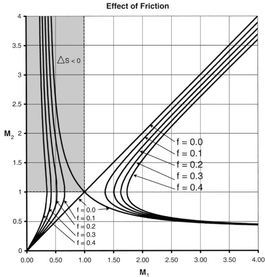
Figure 16.16 Flow in a constant-area duct with friction f as parameter; q = 0 . Upper left quadrant is inaccessible because \Delta S < 0 . \gamma = 1.4 .
