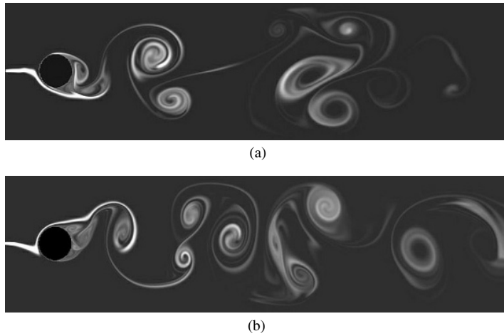
Figure 11.14 Smoke lines in flow around a circular cylinder between two parallel plates at Re = 1000 . The flow geometry is the same as in the fourth example later in this section.
