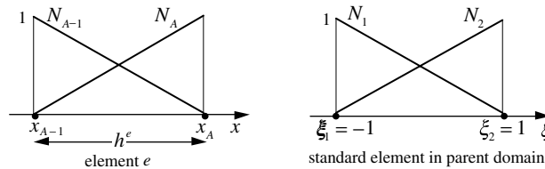
Figure 11.3 Global and local descriptions of an element.
