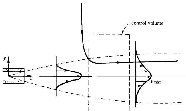
Figure 10.28 Laminar two-dimensional jet. A typical streamline showing entrainment of surrounding fluid is indicated.
