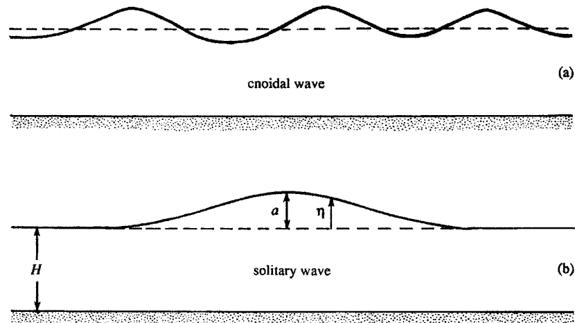
Figure 7.25 Cnoidal and solitary waves. Waves of unchanging form result because nonlinear steepening balances dispersive spreading.
