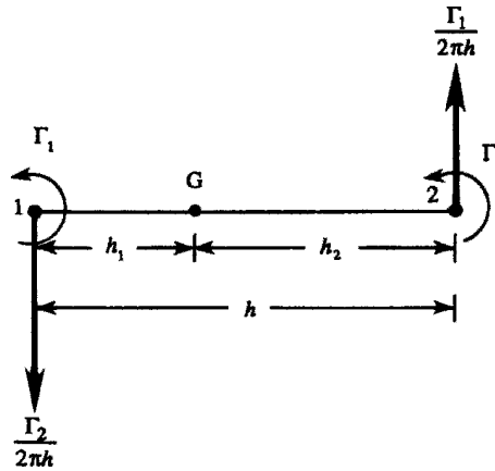
Figure 5.11 Interaction of line vortices of the same sign.
