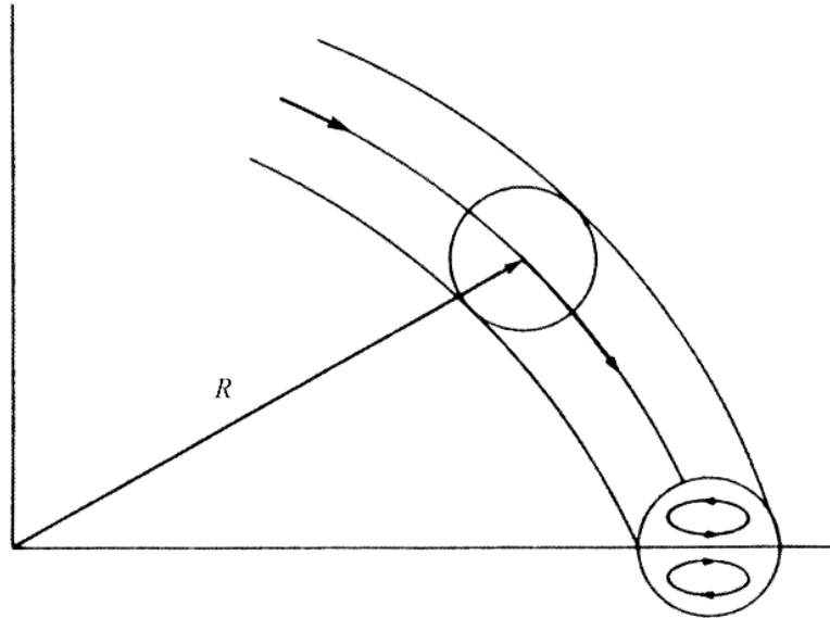
Figure 17.17 Schematic of flow in a curved tube.
