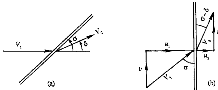
Figure 16.19 (a) Oblique shock wave in which \delta = deflection angle and \sigma = shock angle; and (b) analysis by considering a normal shock and superposing a velocity v parallel to the shock.
