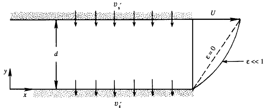
Figure 10.33 Uniform suction in a Couette flow, showing the velocity profile u(y) for \varepsilon = 0 and \varepsilon \ll 1 .
