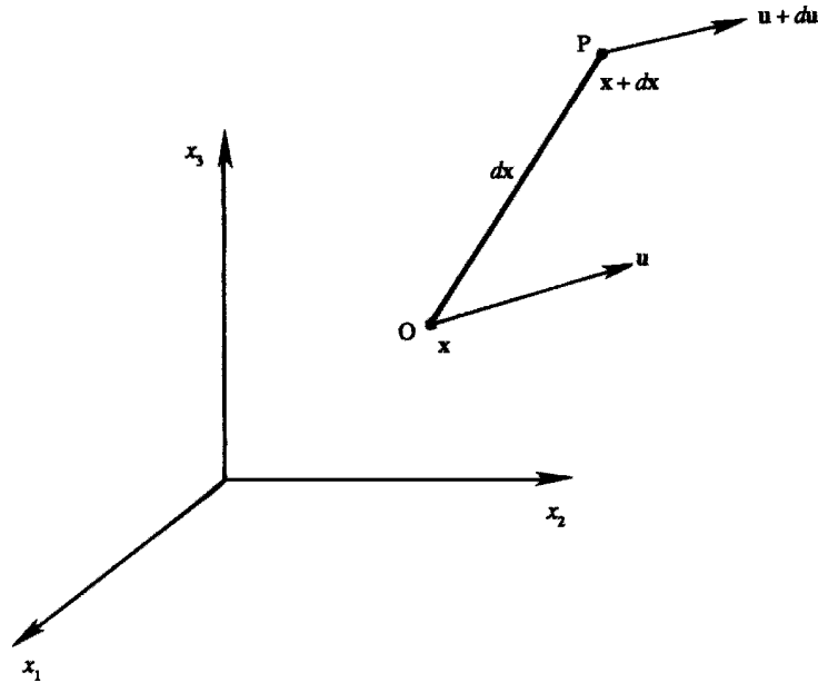
Figure 3.12 Velocity vectors at two neighboring points O and P .
