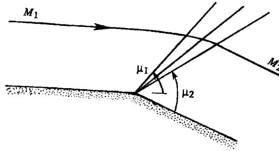
Figure 16.24 The Prandtl-Meyer expansion fan.
