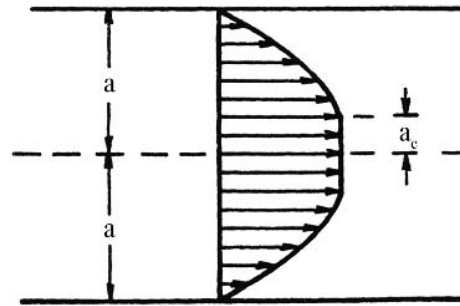
Figure 17.21 Velocity profile for axi-symmetric blood flow in a circular tube.
