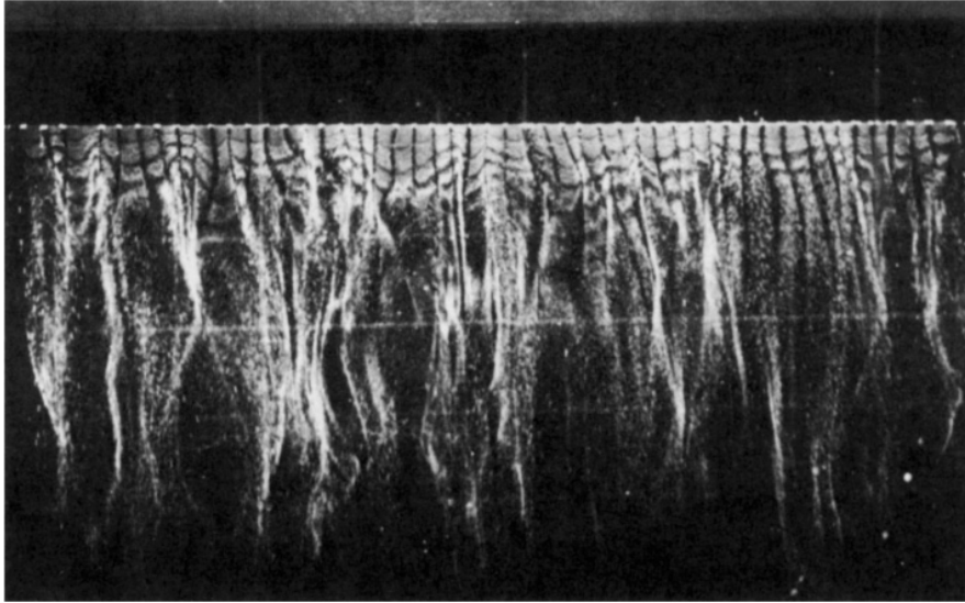
Figure 13.22 Top view of near-wall structure (at y_+ = 2.7 ) in a turbulent boundary layer on a horizontal flat plate. The flow is visualized by hydrogen bubbles. S. J. Kline et al. , Journal of Fluid Mechanics 30 : 741–773, 1967 and reprinted with the permission of Cambridge University Press.
