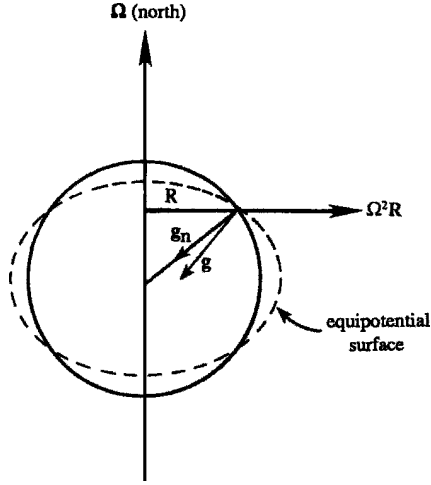
Figure 4.15 Effective gravity \mathbf{g} and equipotential surface.
