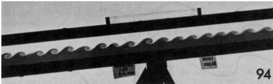
Figure 12.16 Kelvin–Helmholtz instability generated by tilting a horizontal channel containing two liquids of different densities. The lower layer is dyed. Mean flow in the lower layer is down the plane and that in the upper layer is up the plane. S. A. Thorpe, Journal of Fluid Mechanics 46 : 299–319, 1971 and reprinted with the permission of Cambridge University Press.
