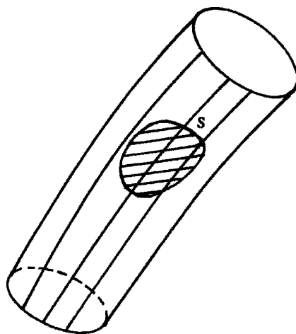
Figure 5.7 Proof of Helmholtz's vortex theorem.
