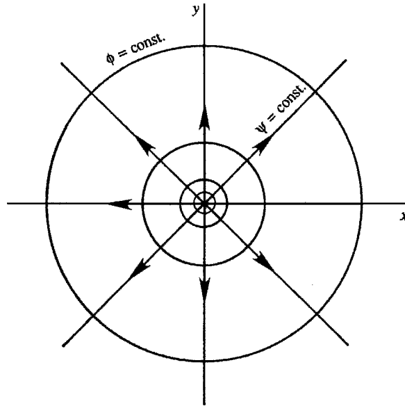
Figure 6.6 Plane source.
