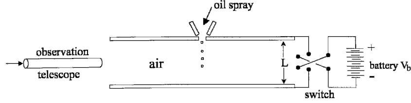
Figure 9.15 Millikan oil drop experiment.
