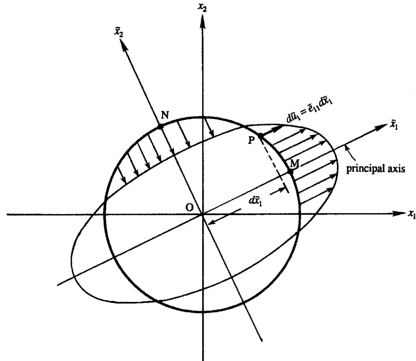
Figure 3.13 Deformation of a spherical fluid element into an ellipsoid.
