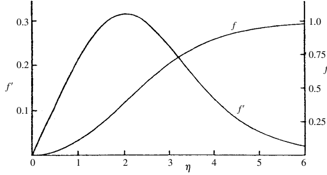
Figure 10.30 Variation of normalized mass flux ( f ) and normalized velocity ( f' ) with similarity variable \eta . Reprinted with the permission of Cambridge University Press.
