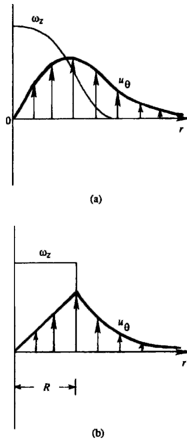
Figure 3.17 Velocity and vorticity distributions in a real vortex and a Rankine vortex: (a) real vortex; (b) Rankine vortex.
