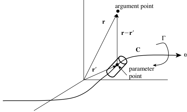
Figure 5.8 Geometry for derivation of Law of Biot and Savart.
