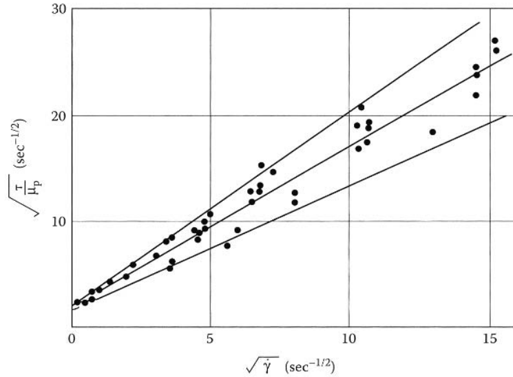
Figure 17.7 Shear stress vs. Shear rate for blood flow. (Reproduced with permission from Whitmore, R. L. (1968) Rheology of Circulation , Pergamon Press, New York).
