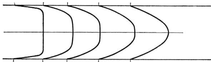
Figure 17.13 Developing velocity profile in a tube flow.
