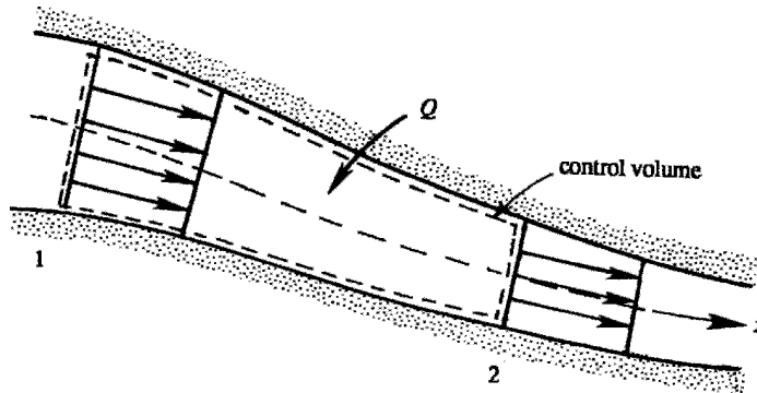
Figure 16.2 A one-dimensional flow.
