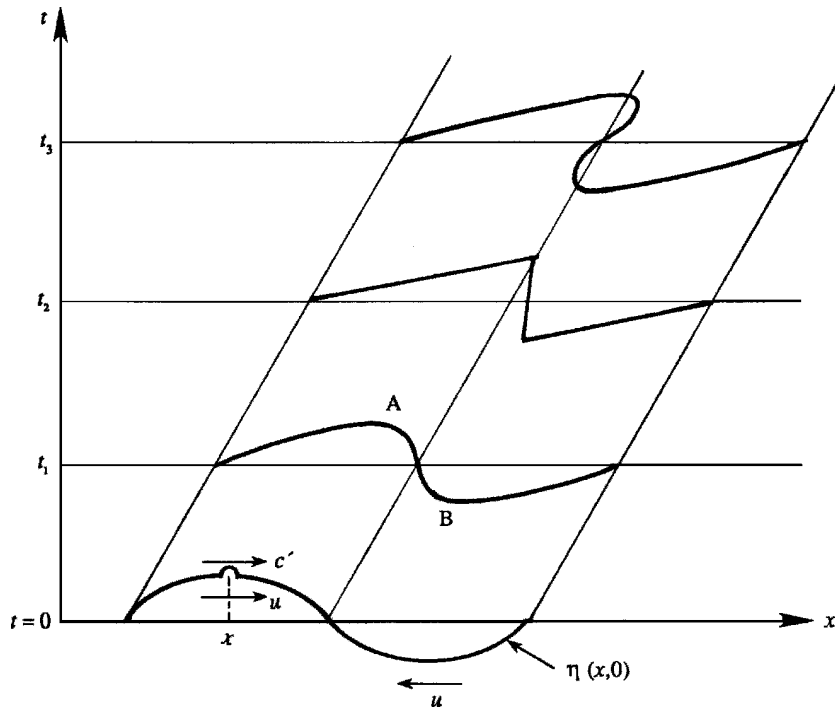
Figure 7.22 Wave profiles at four values of time. At t_2 the profile has formed a hydraulic jump. The profile at t_3 is impossible.
