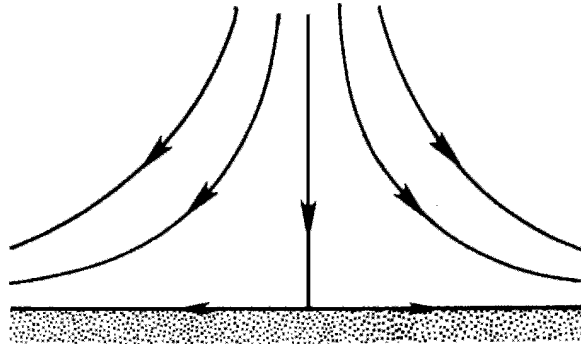
Figure 6.5 Stagnation flow represented by w = Az^2 .
