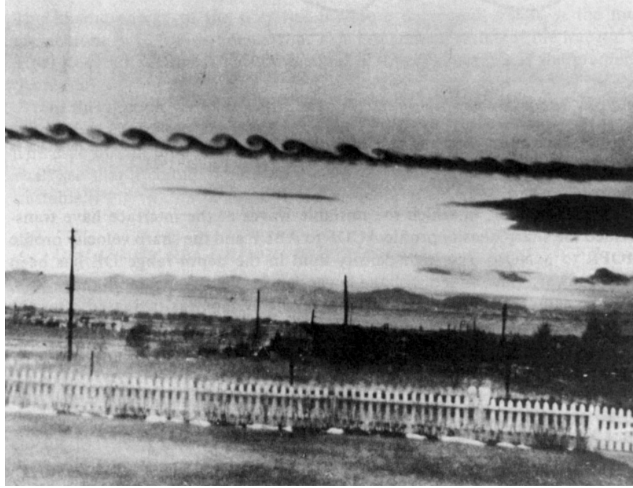
Figure 12.17 Billow cloud near Denver, Colorado. P. G. Drazin and W. H. Reid, Hydrodynamic Stability , 1981 and reprinted with the permission of Cambridge University Press.
