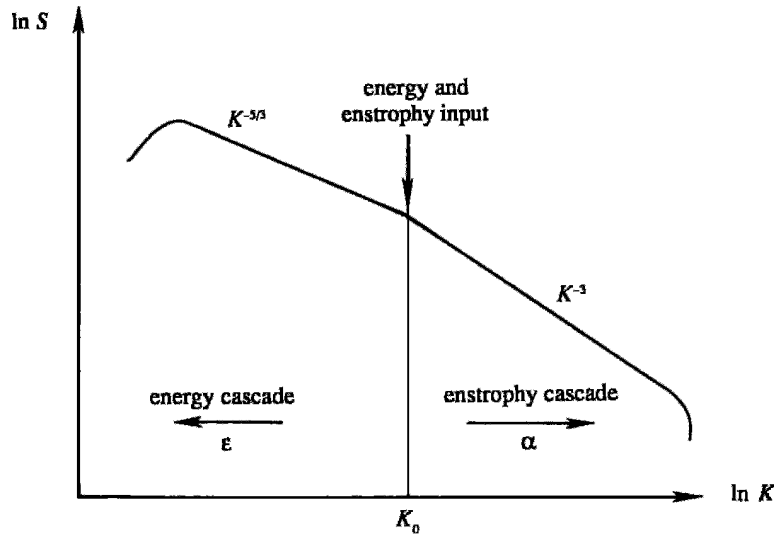
Figure 14.33 Energy and enstrophy cascade in two-dimensional turbulence.
