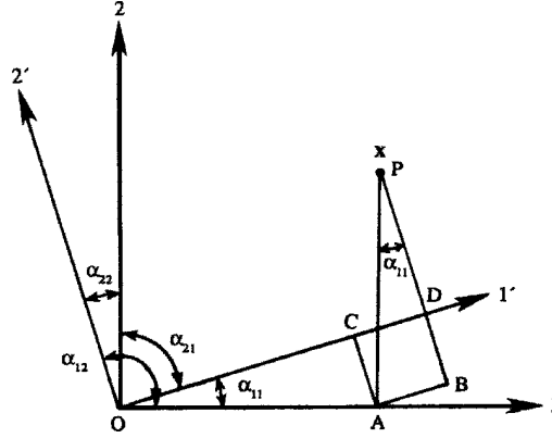
Figure 2.3 Rotation of a coordinate system in two dimensions.
