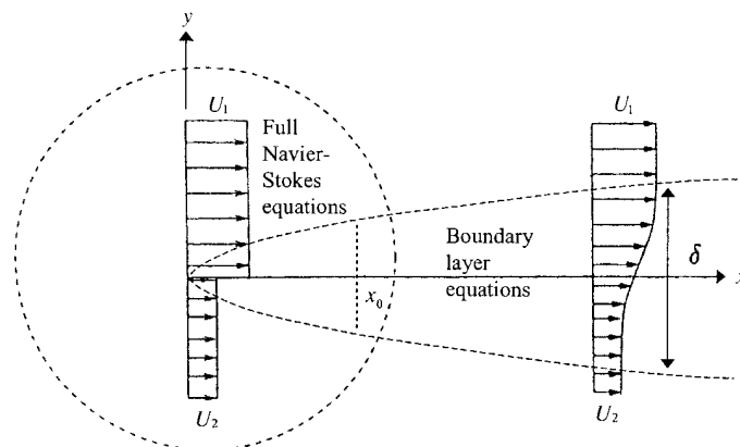
Figure 10.35 Decay of a laminar shear layer.
