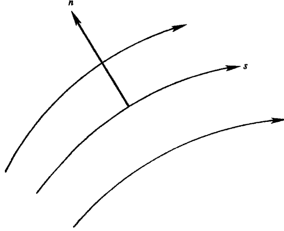
Figure 3.4 Streamline coordinates (s, n) .
