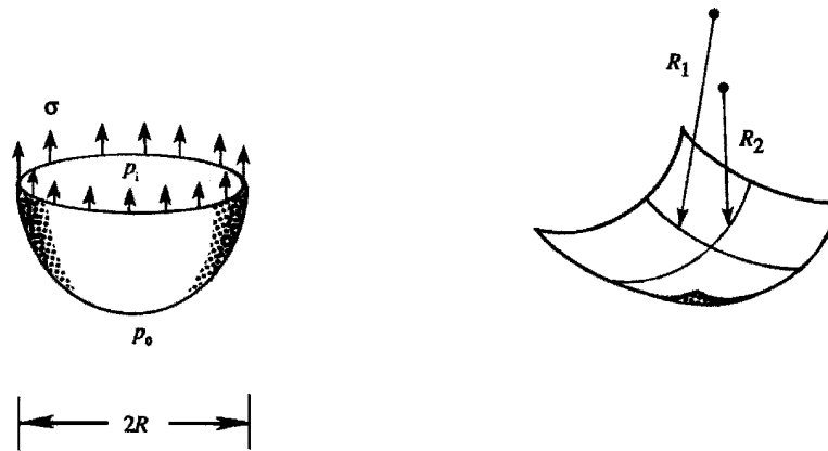
Figure 1.4 (a) Section of a spherical droplet, showing surface tension forces. (b) An interface with radii of curvatures R_1 and R_2 along two orthogonal directions.
