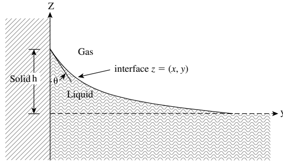
Figure 4.24 Free surface of a liquid adjoining a vertical plane wall.
