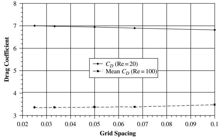
Figure 11.13 Convergence tests for the drag coefficient as the grid spacing decreases. The grid spacing is equal in both directions \Delta x = \Delta y , and time step \Delta t is determined by the stability condition.
