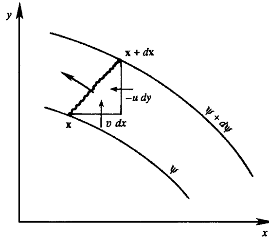
Figure 3.19 Flow through a pair of streamlines.
