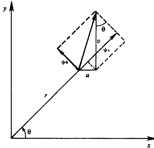
Figure 3.20 Relation of velocity components in Cartesian and plane polar coordinates.
