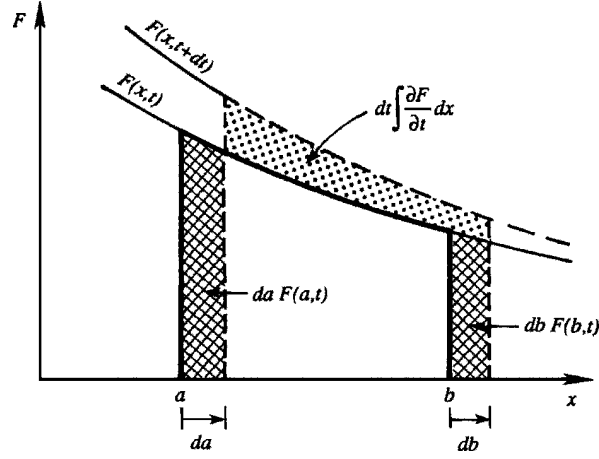
Figure 4.1 Graphical illustration of Leibniz's theorem.
