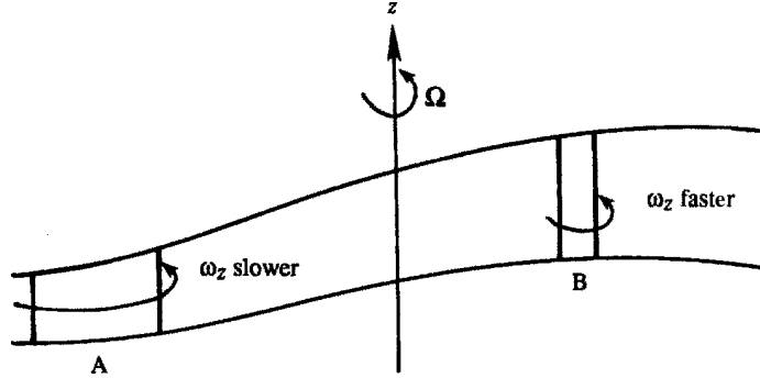
Figure 5.10 Generation of relative vorticity due to stretching of fluid columns parallel to planetary vorticity 2\Omega . A fluid column acquires \omega_z (in the same sense as \Omega ) by moving from location A to location B.
