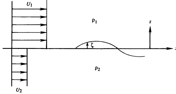
Figure 12.14 Discontinuous shear across a density interface.
