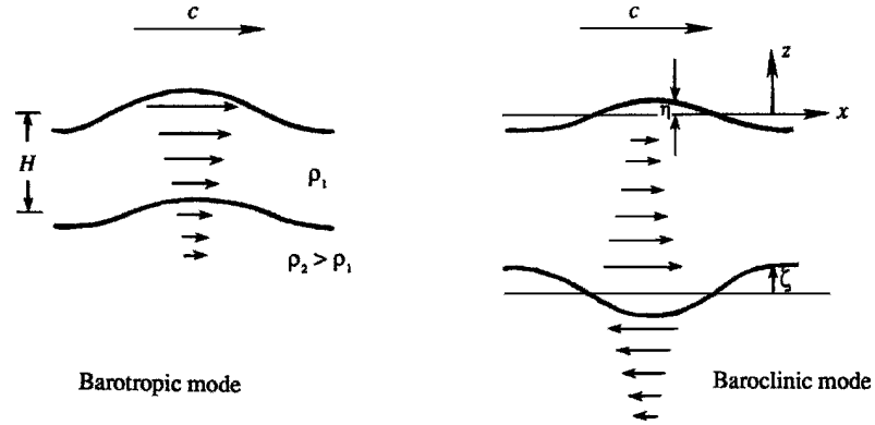
Figure 7.30 Two modes of motion of a layer of fluid overlying an infinitely deep fluid.
