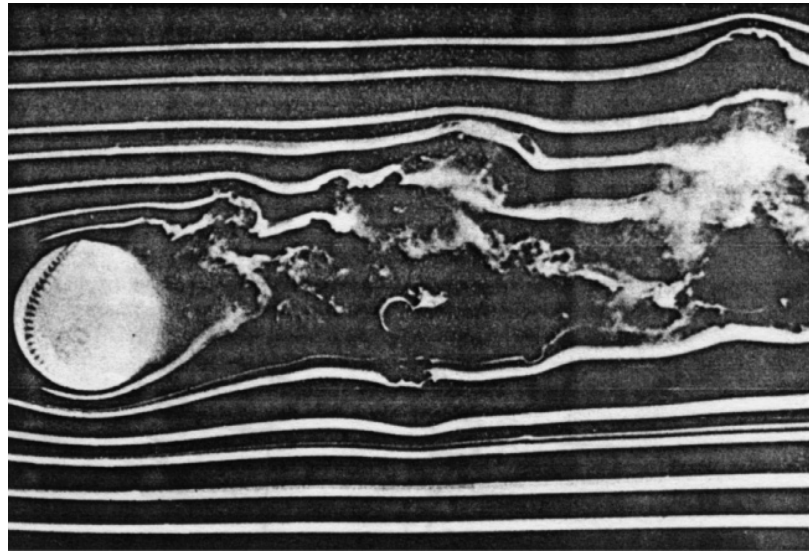
Figure 10.27 Smoke photograph of flow around a spinning baseball. Flow is from left to right, flow speed is 21 m/s, and the ball is spinning counterclockwise at 15 rev/s. [Photograph by F. N. M. Brown, University of Notre Dame.] Photograph reproduced with permission, from the Annual Review of Fluid Mechanics , Vol. 17 © 1985 by Annual Reviews www.AnnualReviews.org .
