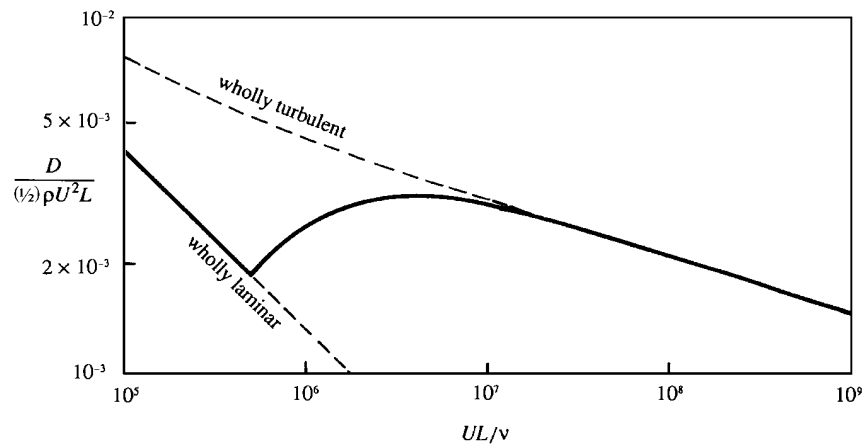
Figure 10.12 Measured drag coefficient for a boundary layer over a flat plate. The continuous line shows the drag coefficient for a plate on which the flow is partly laminar and partly turbulent, with the transition taking place at a position where the local Reynolds number is 5 \times 10^5 . The dashed lines show the behavior if the boundary layer was either completely laminar or completely turbulent over the entire length of the plate.
