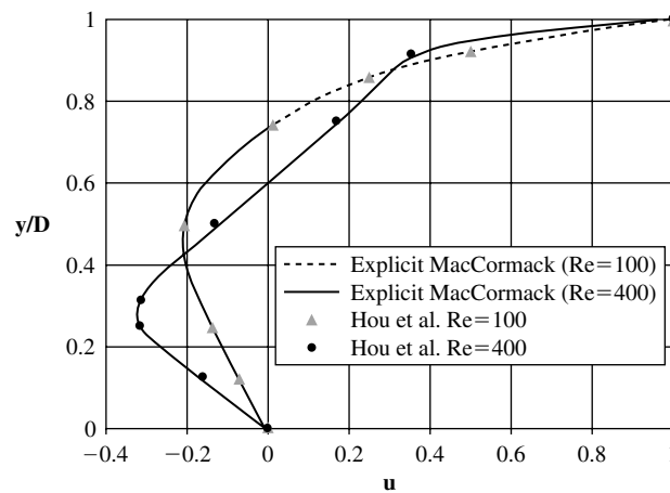
Figure 11.8 Comparison of velocity profiles along a line cut through the center of the cavity ( x = 0.5 D ) at Re = 100 and 400.
