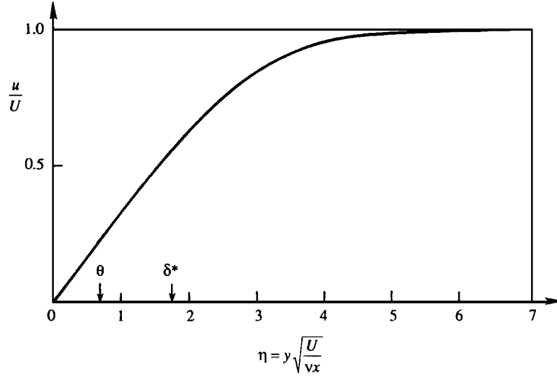
Figure 10.7 The Blasius similarity solution of velocity distribution in a laminar boundary layer on a flat plate. The momentum thickness \theta and displacement \delta^* are indicated by arrows on the horizontal axis.
