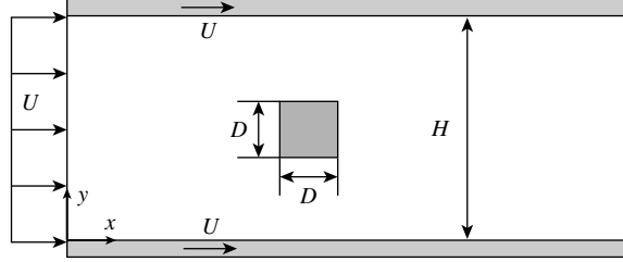
Figure 11.9 Flow around a square block between two parallel plates.
