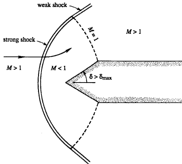
Figure 16.22 Detached shock.
