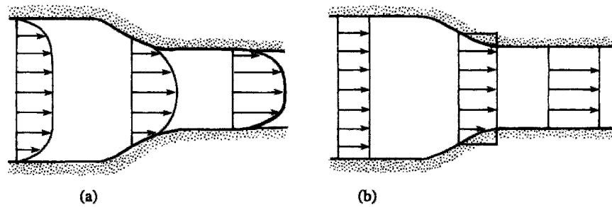
Figure 3.18 Flow through a conduit and its one-dimensional approximation: (a) real flow; (b) one-dimensional approximation.
