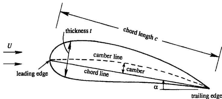
Figure 15.6 Airfoil geometry.
