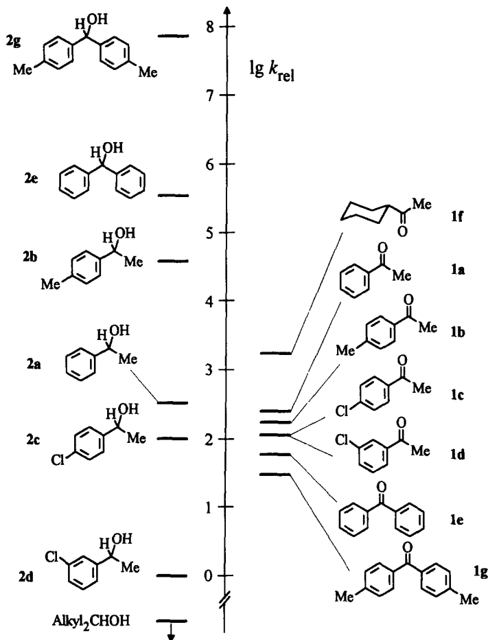
Scheme 4. Relative reactivities of ketones and alcohols in ionic hydrogenations ( \text{CF}_3\text{CO}_2\text{H}/\text{Et}_3\text{SiH} ).
