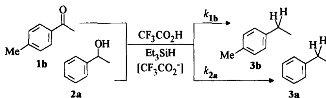
Scheme 2. Competition experiment to determine \kappa = k_{2a}/k_{1b}
