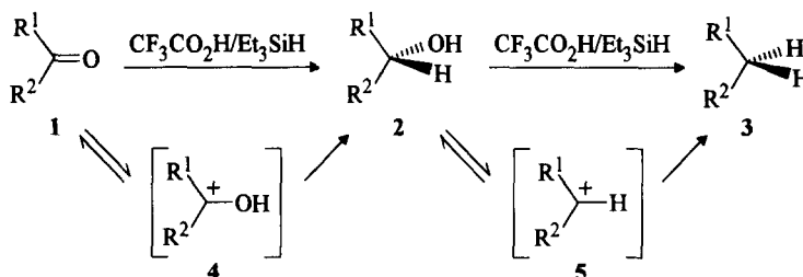
Scheme 1. Ionic hydrogenations of ketones and alcohols
