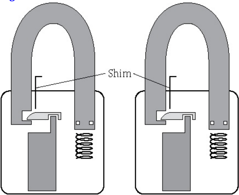
Figure 7-8 : How a shim works.
