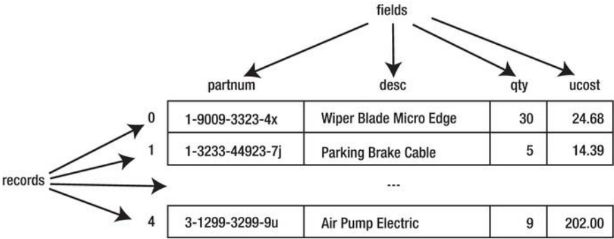
Figure 8-1. This flat file database describes automotive parts.
