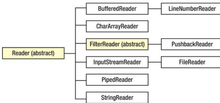
Figure 8-8. Unlike FilterInputStream , FilterReader is abstract.
