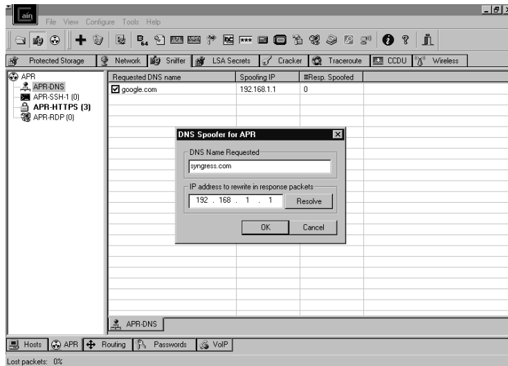
Figure 8.7 Adding a New DNS Spoofer Target in Cain
