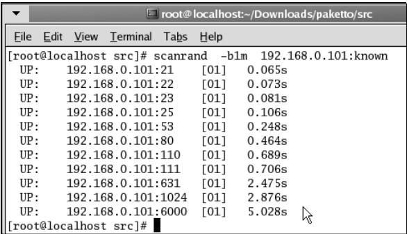
Figure 5.13 Sample Scanrand Result
