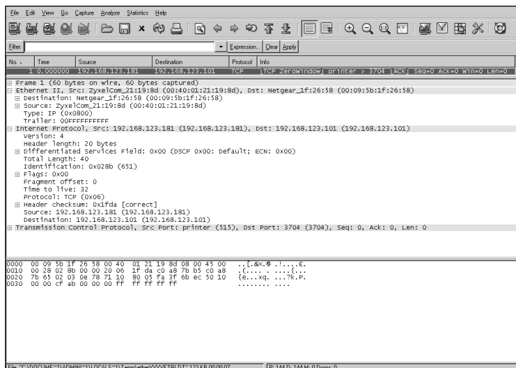
Figure 4.2 IP Ethernet Capture
