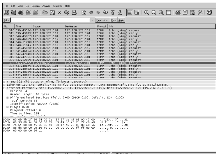
Figure 4.21 Ptunnel
