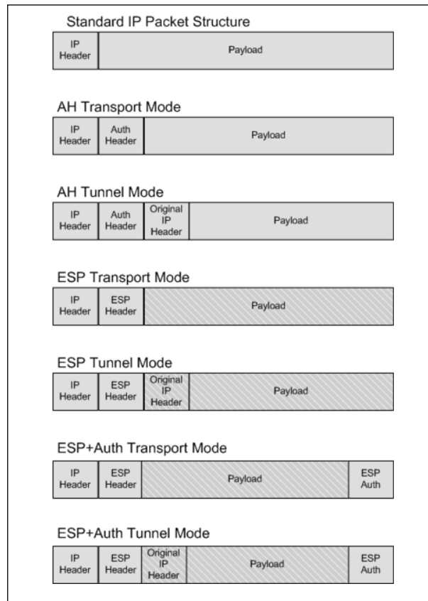
Figure 7.22 Packet Structure Comparison
