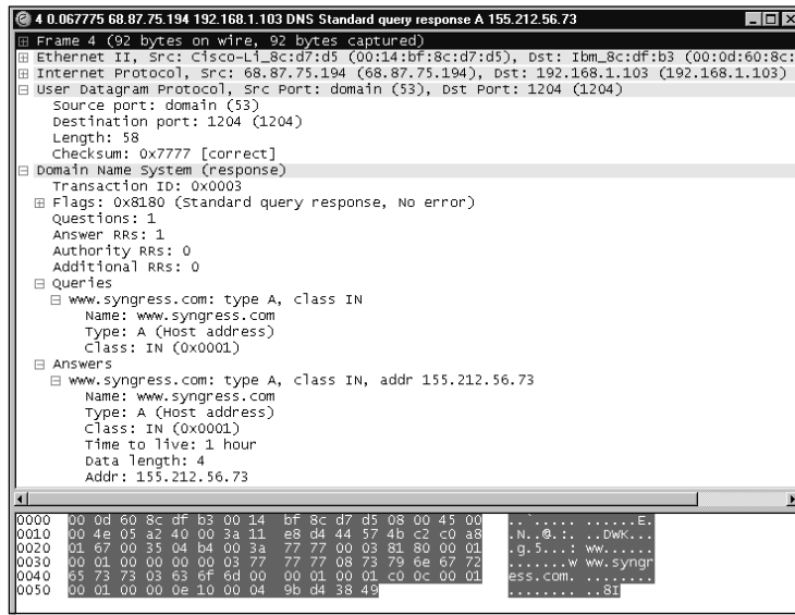
Figure 8.2 Ethernet Capture of a DNS Response
