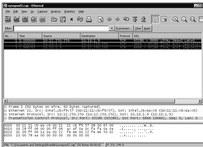
Figure 6.2 Spoofing the Source Address of a SYN Packet
