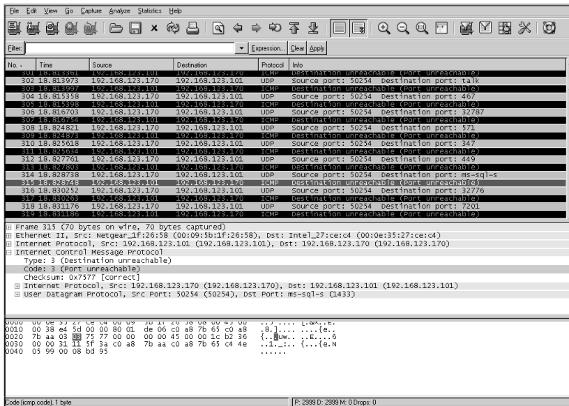
Figure 4.19 Port Scan
