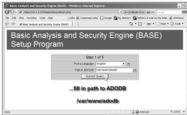
Figure 5.33 Configure BASE
