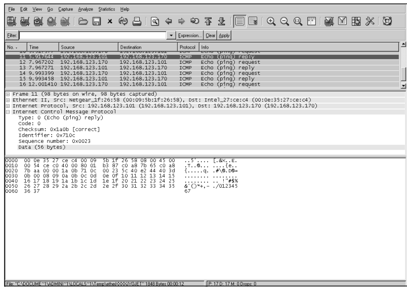
Figure 4.17 Linux Ping
