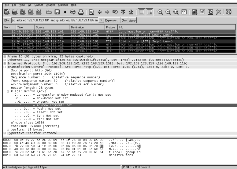
Figure 4.22 ACKCMD
