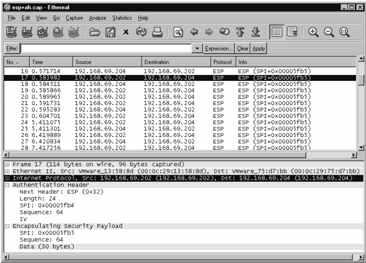
Figure 7.21 Ethereal Capture of ESP+AH Packets
