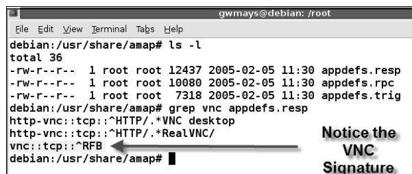
Figure 5.11 Sample Amap Response Matching Pattern
