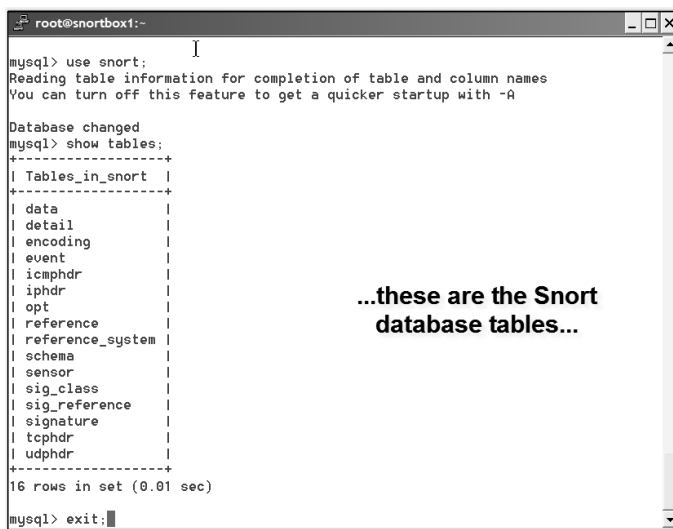
Figure 5.32 Snort Database Setup
