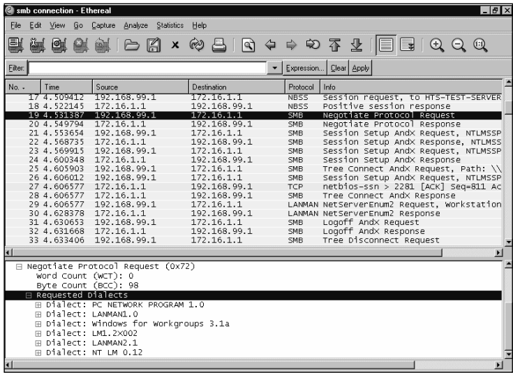
Figure 7.1 Ethernet Capture of SMB Connection
