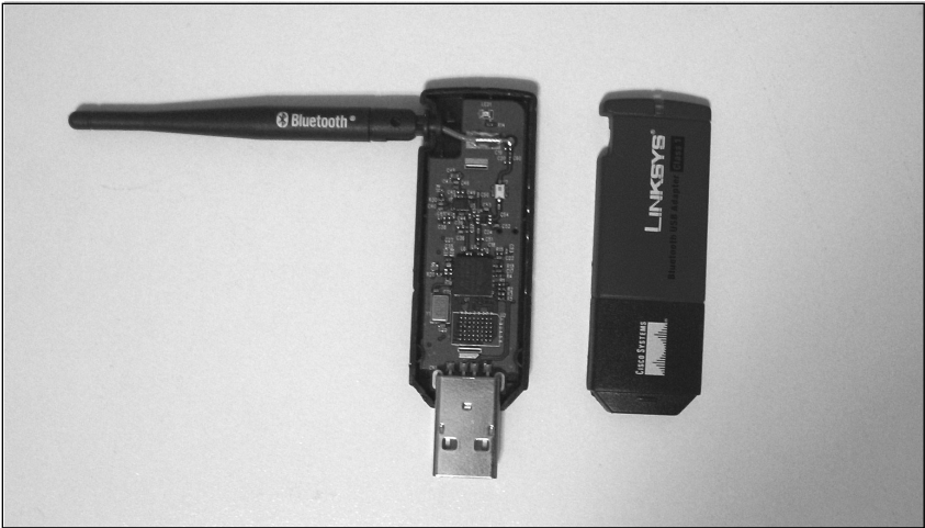
Figure 2.10 Opening the Bluetooth Adapter Case
