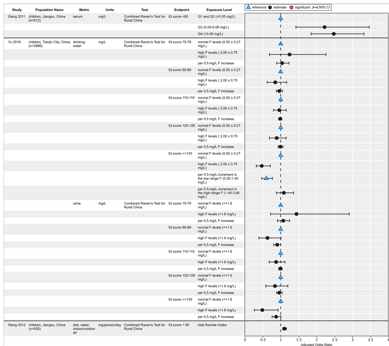
Figure D5. IQ Score in Children by Fluoride Exposure (low risk-of-bias studies; presented as adjusted OR)
