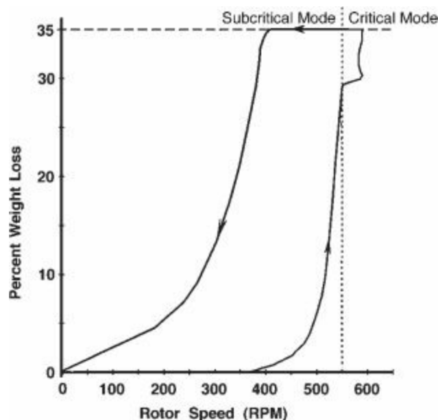
Figure 10.7. Weight loss as a function of rotor speed when a 20-kilovolt potential was applied
