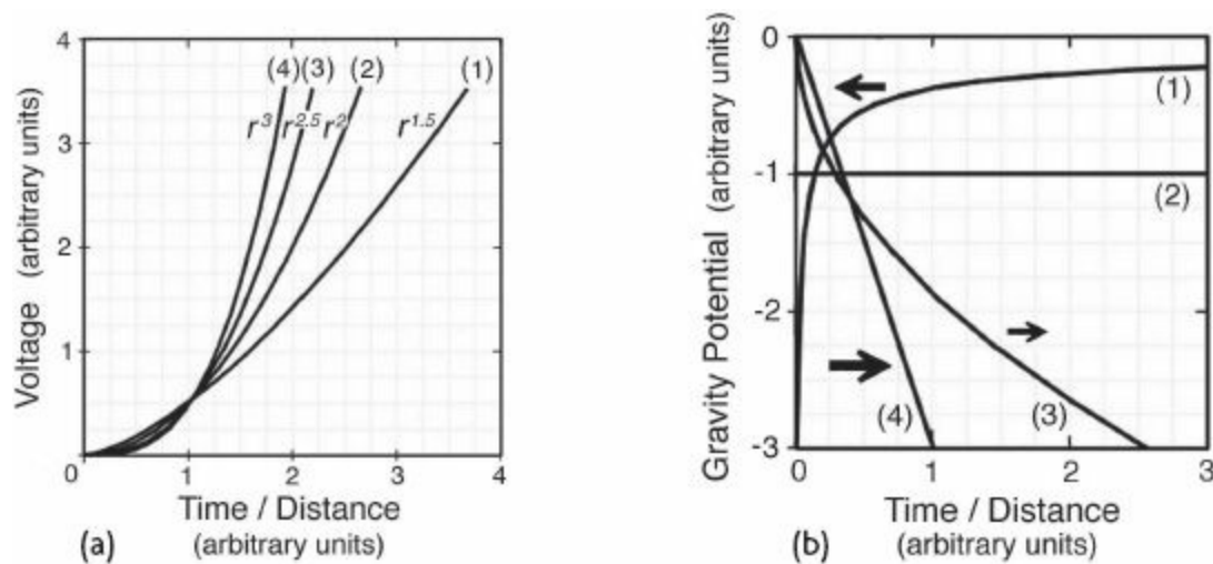
Figure 7.7. (a) Leading-edge profiles for waves whose voltage rises exponentially with varying degrees of nonlinearity, as: r^{1.5} (curve 1), r^2 (curve 2), r^{2.5} (curve 3), and r^3 (curve 4). (b) Corresponding gravity potential distribution generated by the resulting virtual-charge distribution. (P. LaViolette, © 2007)
