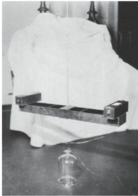
Figure 1.3. An experimental setup designed to measure the thrust produced by Thomas Townsend Brown's gravitators. (Photo courtesy of the Townsend Brown Family and Qualight, L.L.C.)
