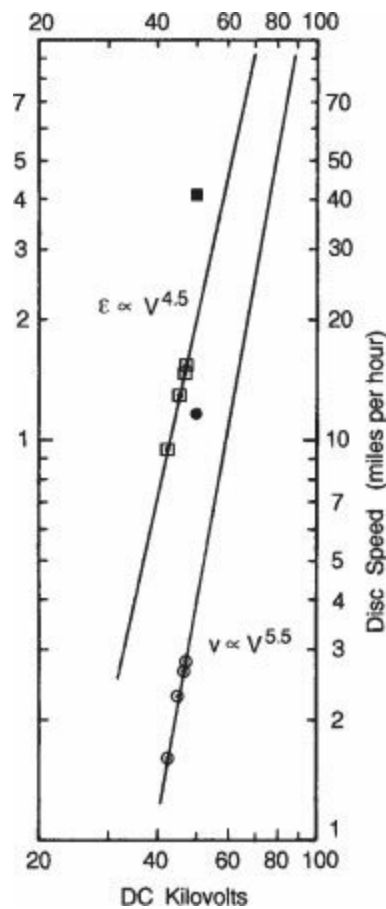
Figure 2.4. A logarithmic plot showing how the velocity (right line) and efficiency (left line) of Thomas Townsend Brown's electrogravitic discs increased with voltage. Empty squares and circles indicate the ONR measurements of the 1.5-foot-diameter discs, while solid squares and circles indicate the performance of an improved 2-foot-diameter model. (P. LaViolette, © 1997)
