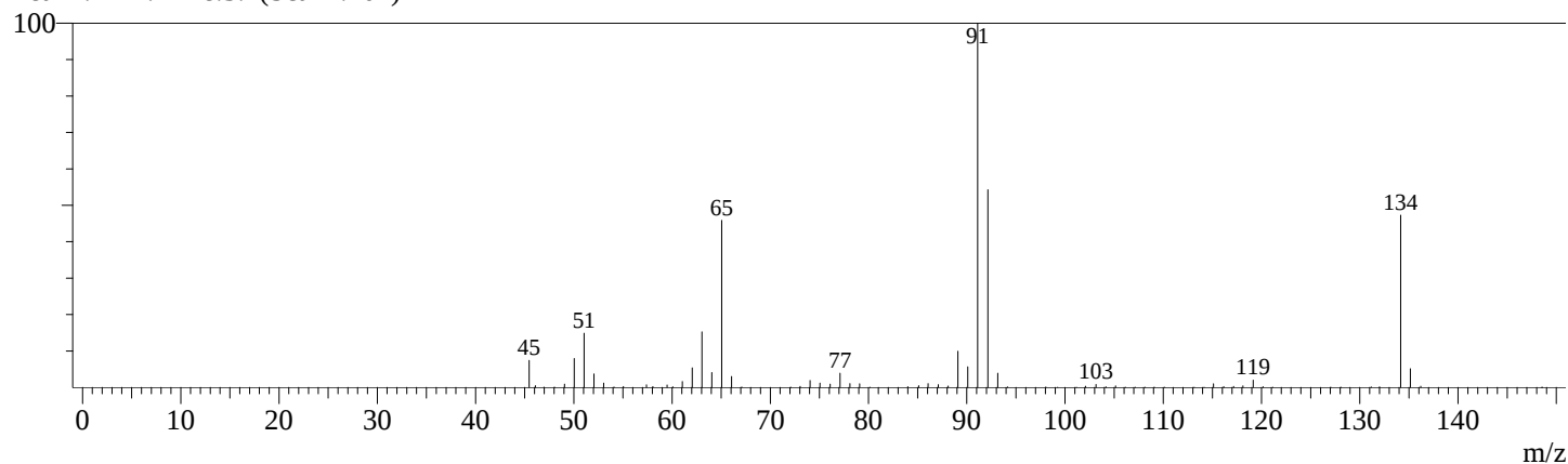
Peak#:2 R.Time:6.4(Scan#:465)
