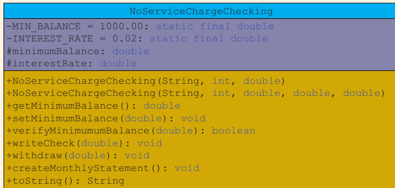
FIGURE 10-11 UML class diagram of the class NoServiceChargeChecking
