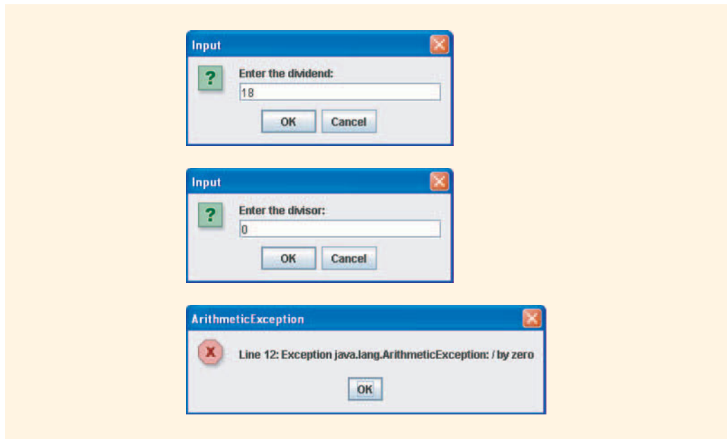
FIGURE 11-6 Sample Run 2 of the program ExceptionExample4
