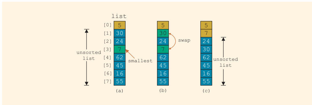
FIGURE 14-4 Elements of list during the second iteration
