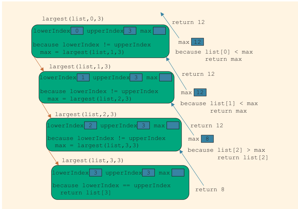
FIGURE 13-4 Execution of largest(list, 0, 3)
