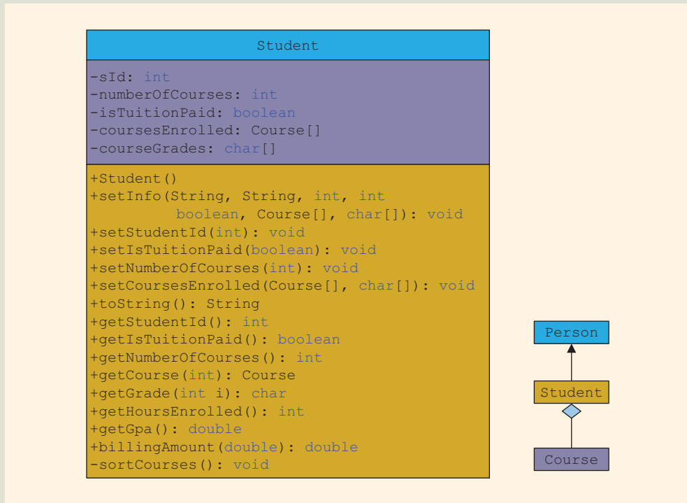
FIGURE 10-19 UML class diagram of the class Student
