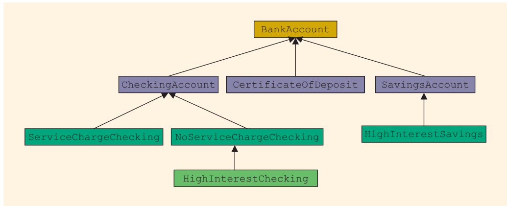
FIGURE 10-7 Inheritance hierarchy of banking accounts
