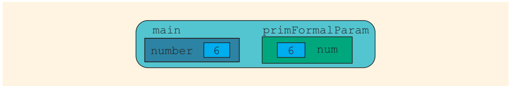
FIGURE 7-4 The variables number and num before execution of the statement in Line 13
