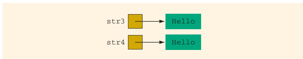
FIGURE 4-8 Variables str3 , str4 , and the objects to which they point
