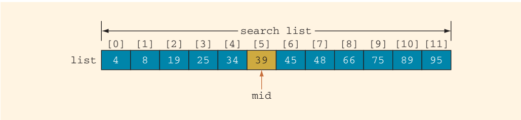
FIGURE 14-20 Search list, list[0]...list[11]
