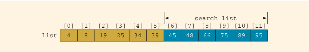
FIGURE 14-21 Search list, list[6]...list[11]
