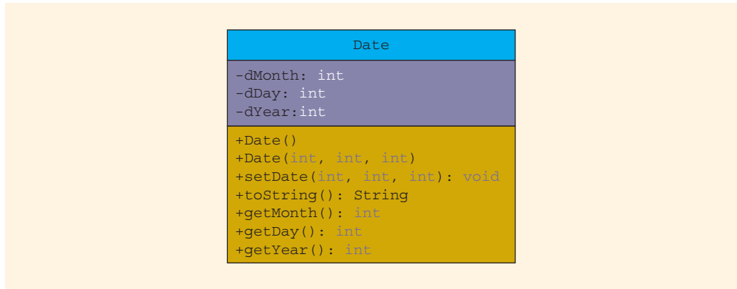
FIGURE 10-16 UML class diagram of the class Date
