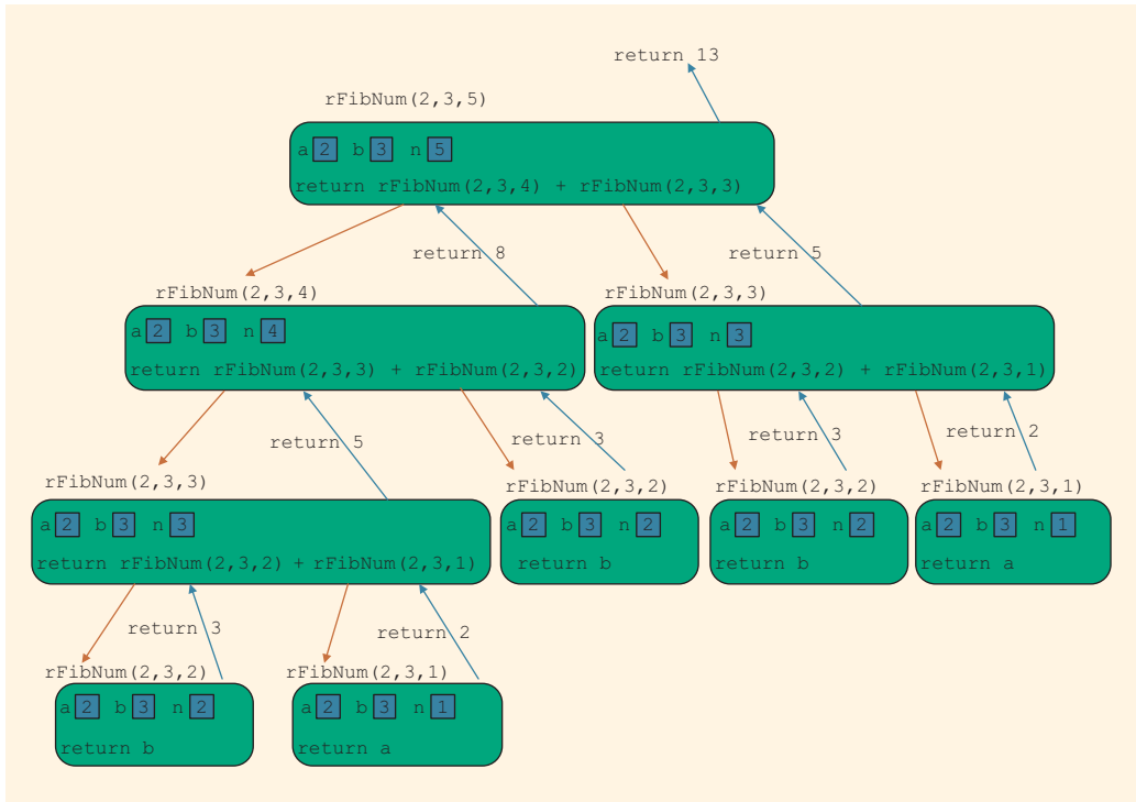
FIGURE 13-5 Execution of rFibNum(2, 3, 5)
