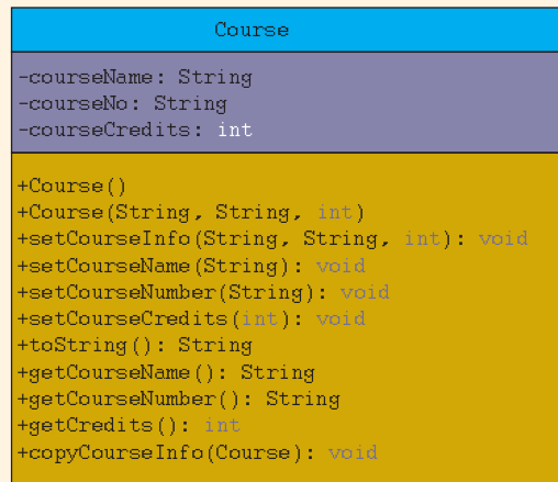
FIGURE 10-18 UML class diagram of the class Course
