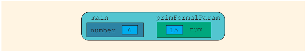
FIGURE 7-5 The variables number and num after execution of the statement in Line 13
