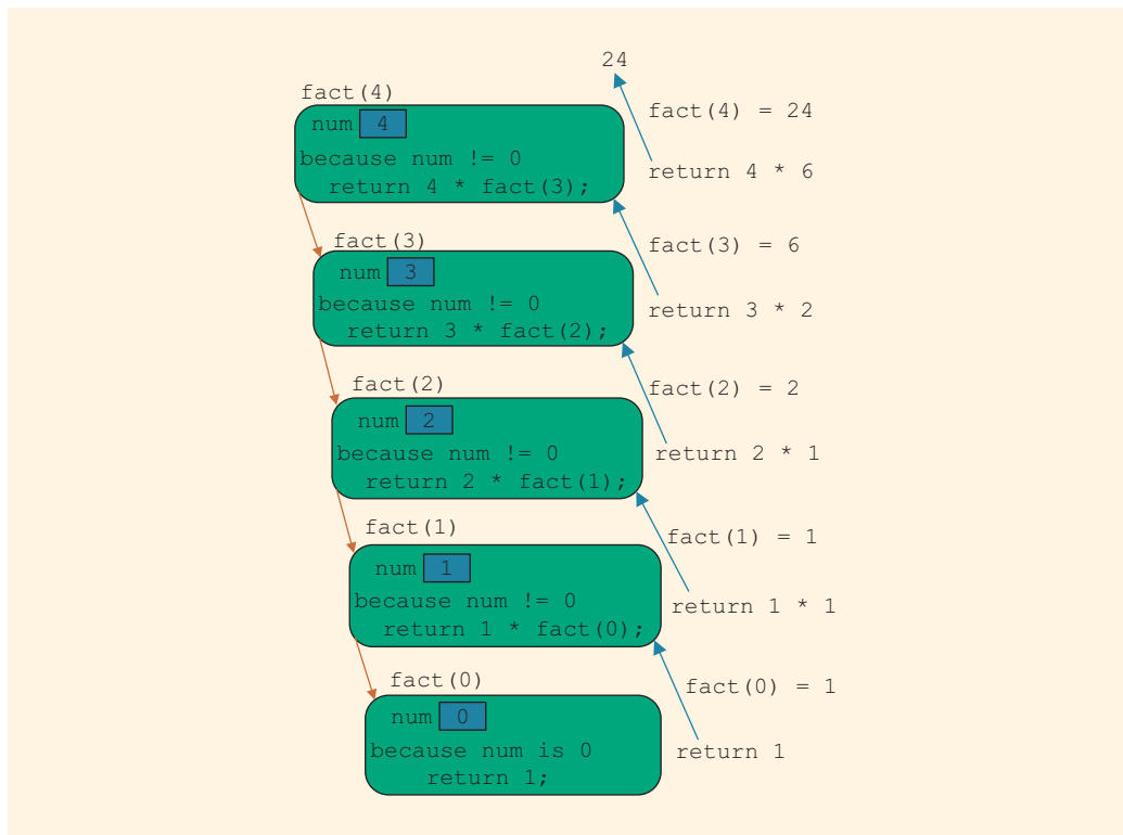
FIGURE 13-1 Execution of fact(4)
