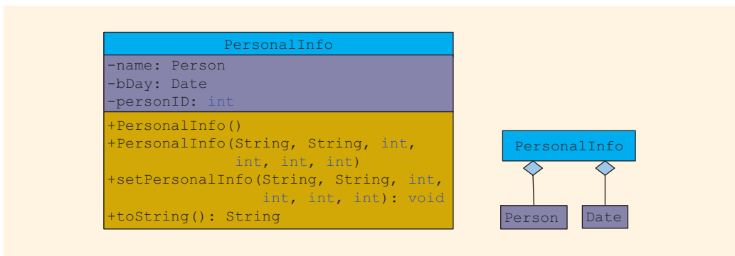
FIGURE 10-17 UML class diagram of the class PersonalInfo
