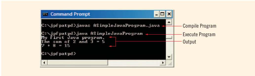
FIGURE D-14 Compiling and executing the program ASimpleJavaProgram.java
