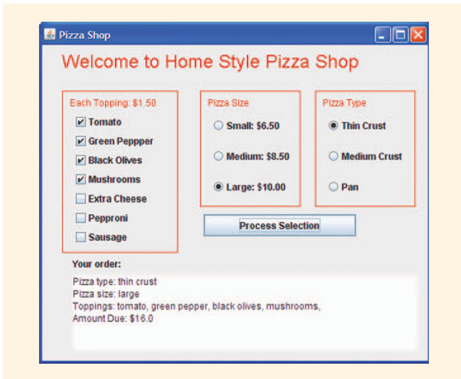
FIGURE 12-32 Figure for Programming Exercise 19
