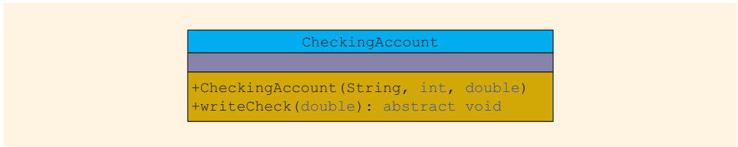
FIGURE 10-9 UML class diagram of the class CheckingAccount
