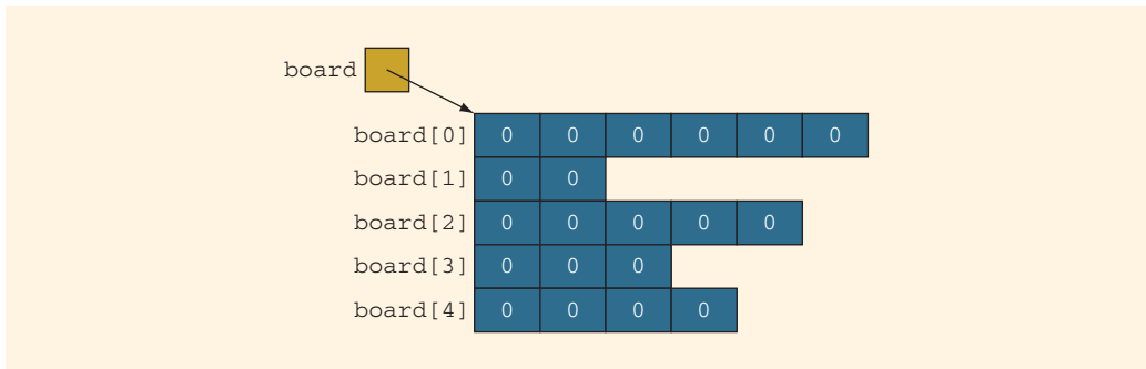
FIGURE 9-18 Array board
