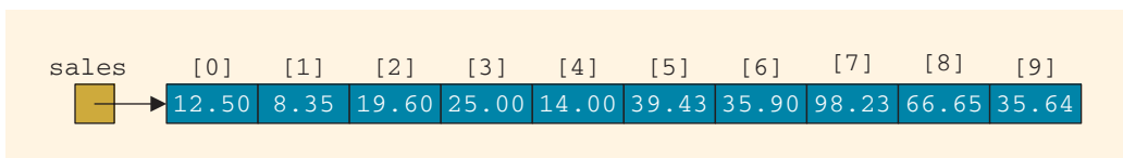
FIGURE 9-6 Array sales
