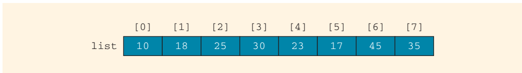
FIGURE 14-5 List
