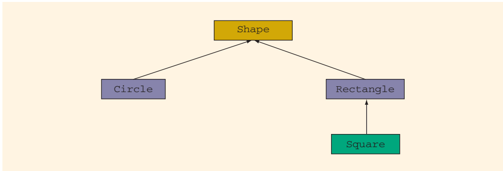
FIGURE 10-1 Inheritance hierarchy
