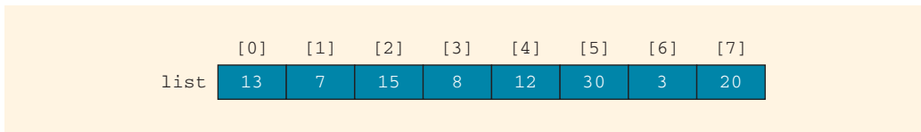
FIGURE 14-12 Unsorted list
