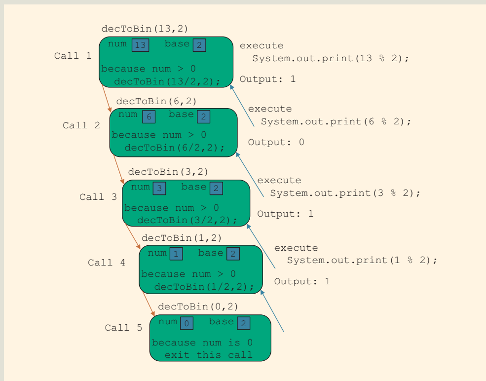
FIGURE 13-8 Execution of decToBin(13, 2)
