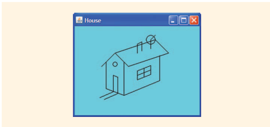
FIGURE 12-31 House
