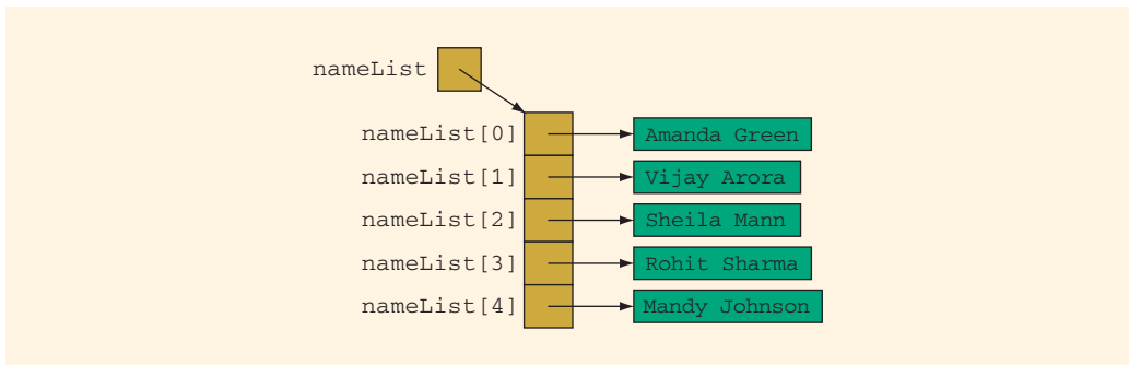
FIGURE 9-11 Array nameList
