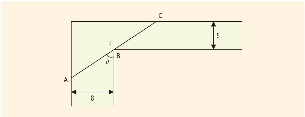
FIGURE 7-19 Pipe problem
