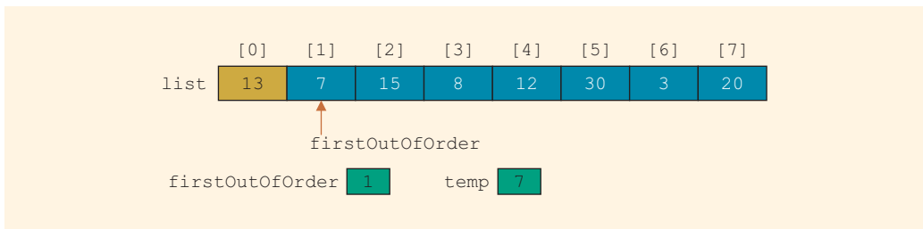
FIGURE 14-13 firstOutOfOrder = 1
