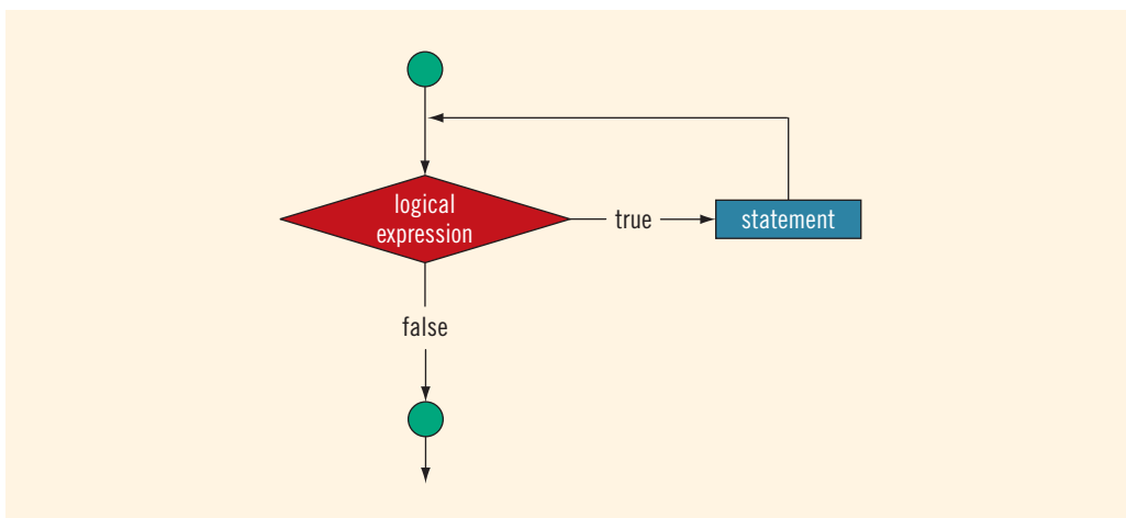
FIGURE 5-1 while loop
