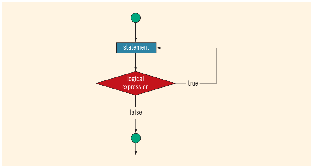
FIGURE 5-5 do...while loop
