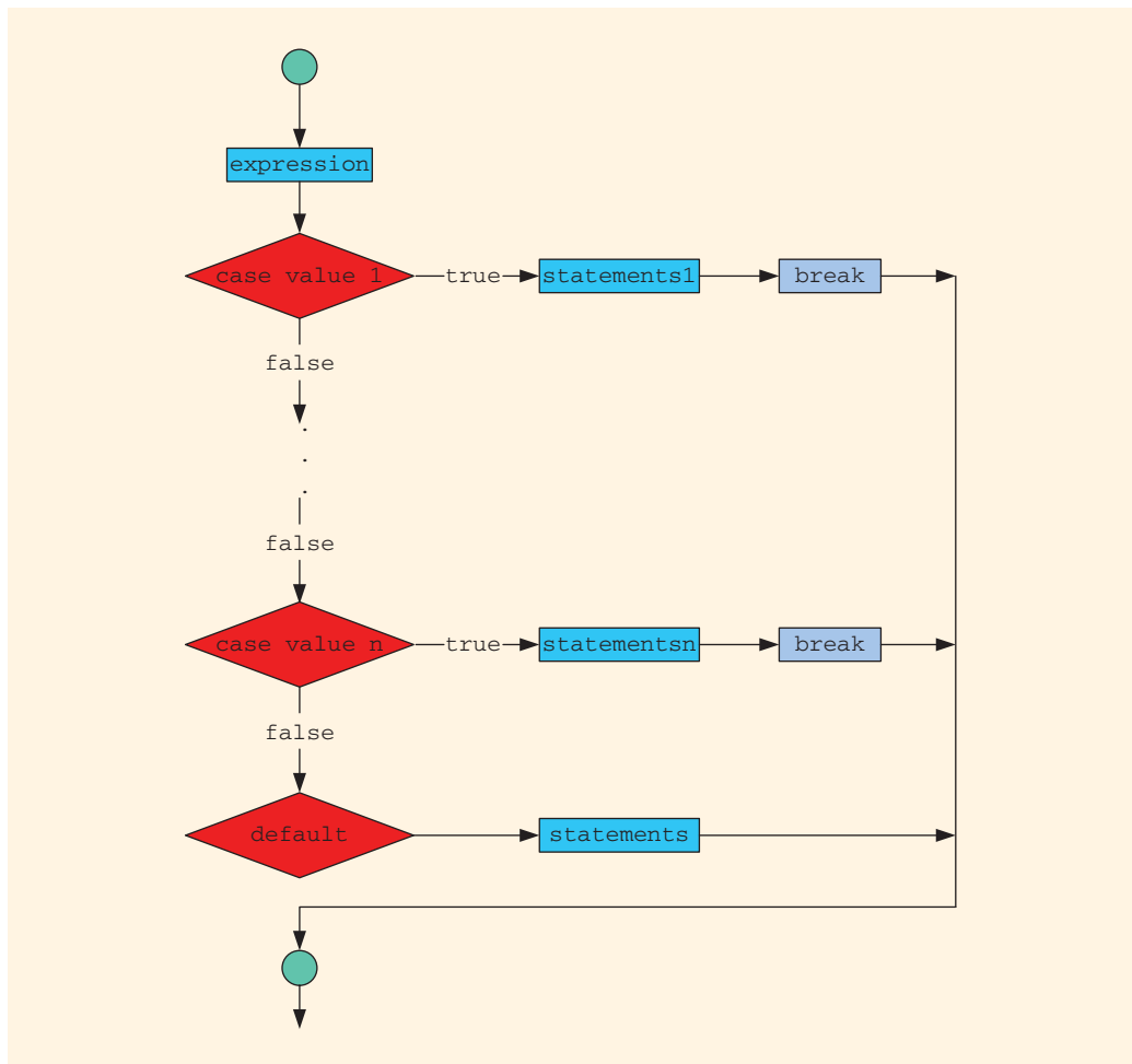
FIGURE 4-5 switch statement
