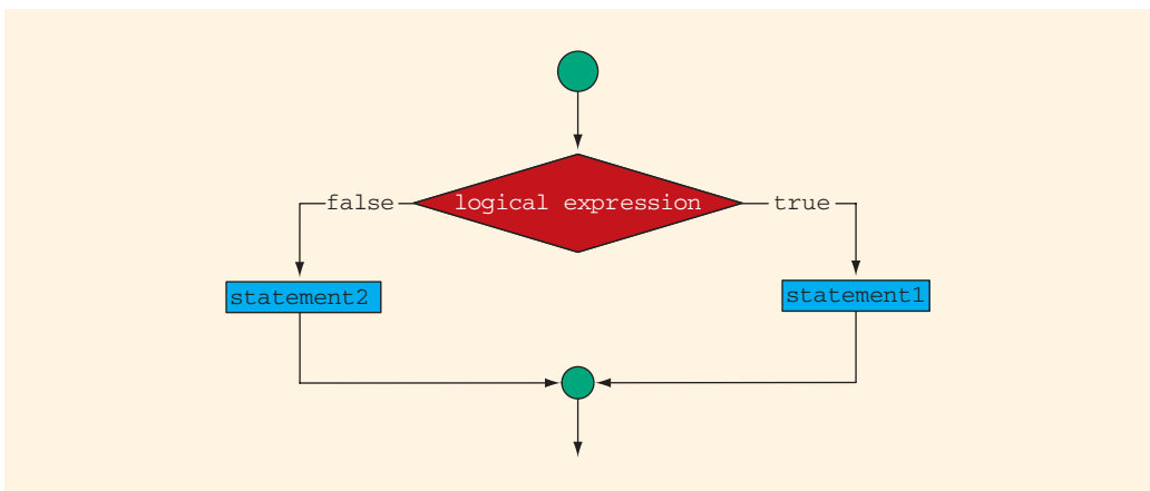
FIGURE 4-4 Two-way selection
