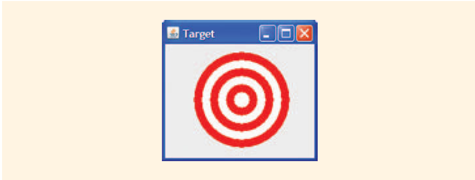
FIGURE 12-30 Target practice
