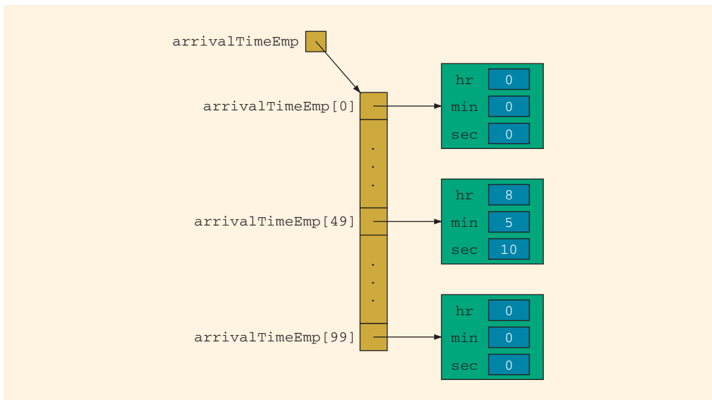
FIGURE 9-14 Array arrivalTimeEmp after setting the time of employee 49
