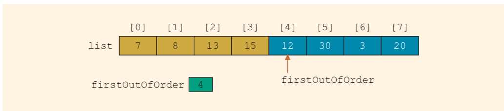
FIGURE 14-15 First out-of-order element is at position 4
