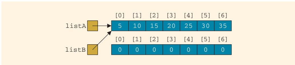
FIGURE 9-8 Arrays after the statement listB = listA ; executes
