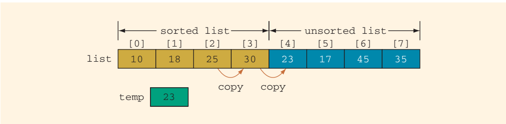
FIGURE 14-9 List before copying list[3] into list[4] , and then list[2] into list[3]
