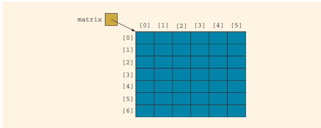
FIGURE 9-21 Two-dimensional array matrix
