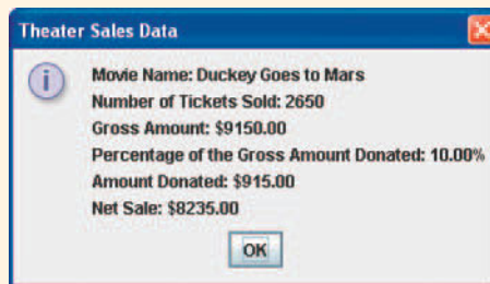
FIGURE 3-14 Output of theater sales program
