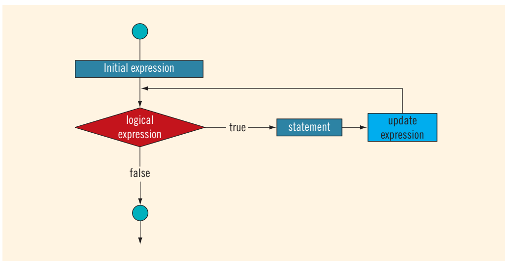
FIGURE 5-4 for loop
