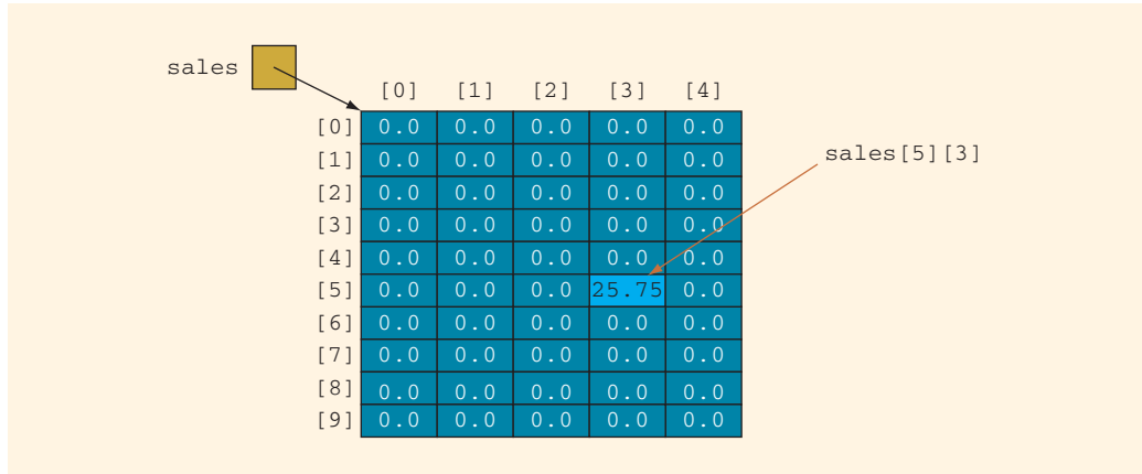
FIGURE 9-17 sales[5][3]
