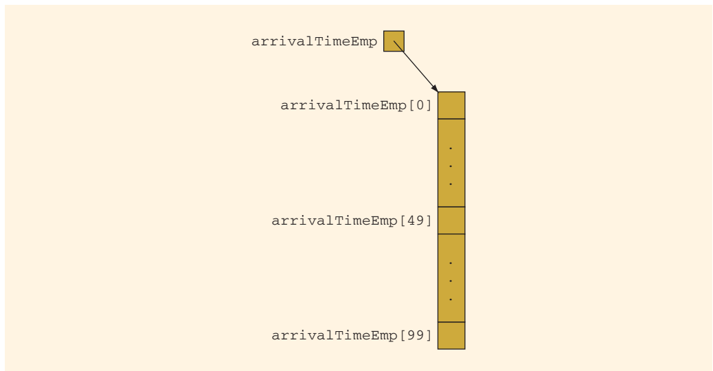
FIGURE 9-12 Array arrivalTimeEmp
