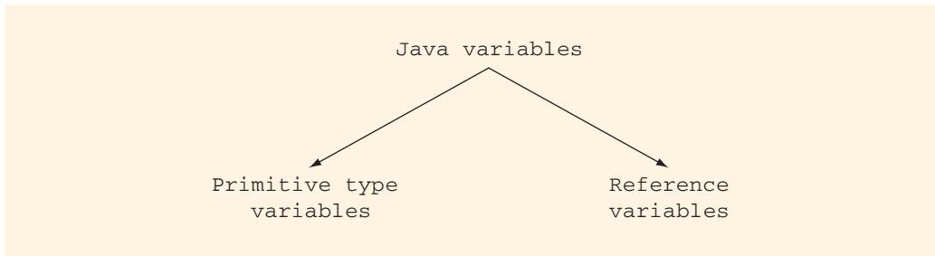
FIGURE 3-6 Java variables
