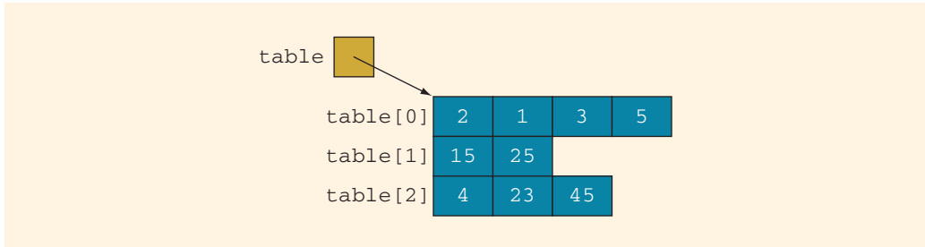
FIGURE 9-20 Array table
