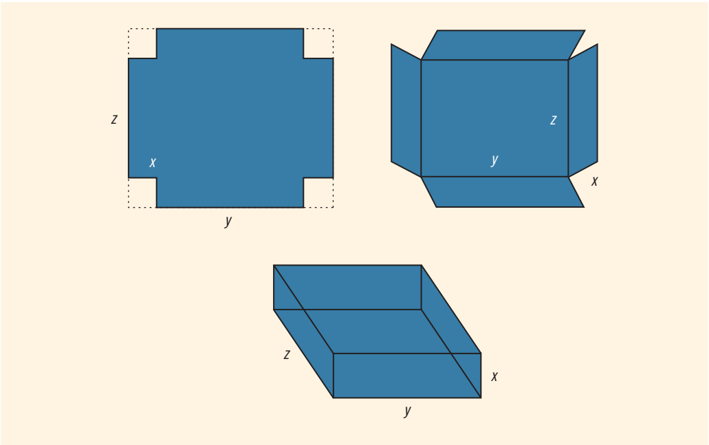
FIGURE 7-17 Cardboard box
