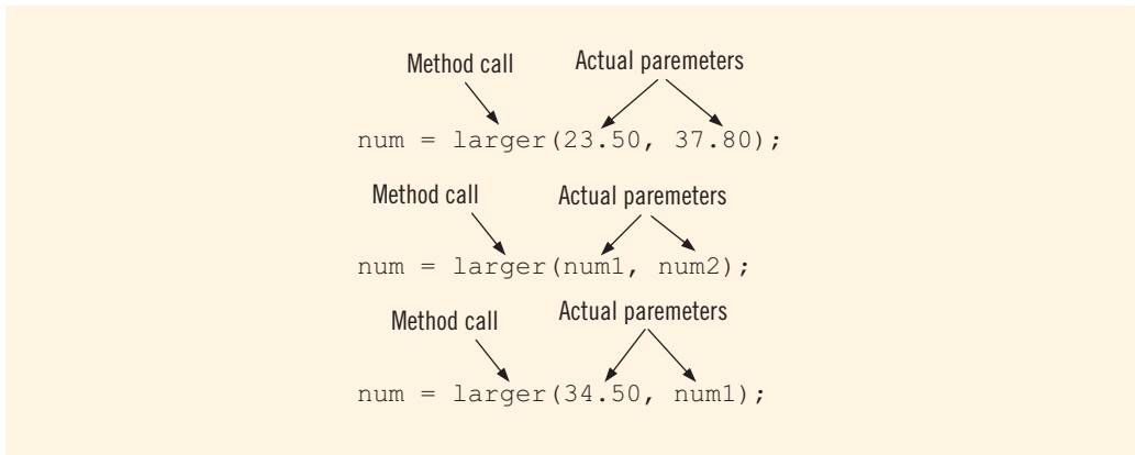
FIGURE 7-2 Method calls
