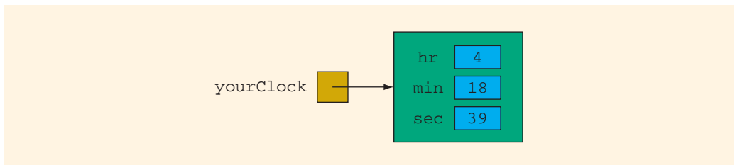
FIGURE 8-11 Object yourClock
