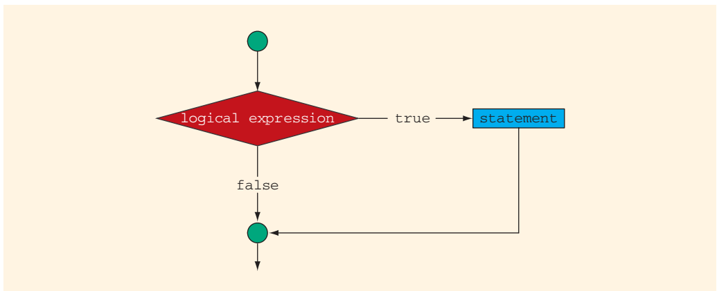
FIGURE 4-2 One-way selection
