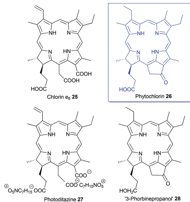
Fig. 12 Chlorin type photosensitizers derived from natural sources.
