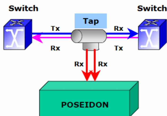
Figure 15: ELAMAN's POSEIDON Internet Monitoring Centre connected with a tap to the network (source Privacy International 323 )
