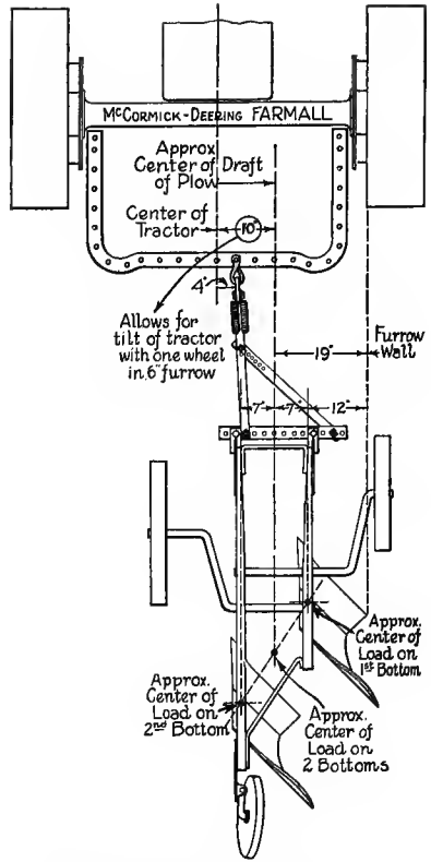
Illust. 36. Shows 2-bottom plow (14-inch bottoms) hitched to the Farmall.
