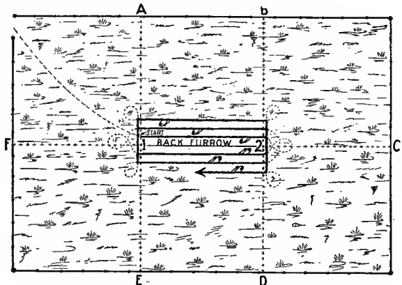
Illust. 47. Method sometimes practiced alternately with that shown in Illust. 45. Points 1 and 2 located as in Illust. 44 and a land back-furrowed a few rounds after which furrows are plowed across ends, complete turn made at corners by looping to left.
