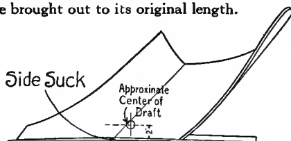
Illust. 39. Top view of a plow bottom showing side suck. The side suck varies from \frac{1}{8} to \frac{1}{4} inch in plow bottoms.
