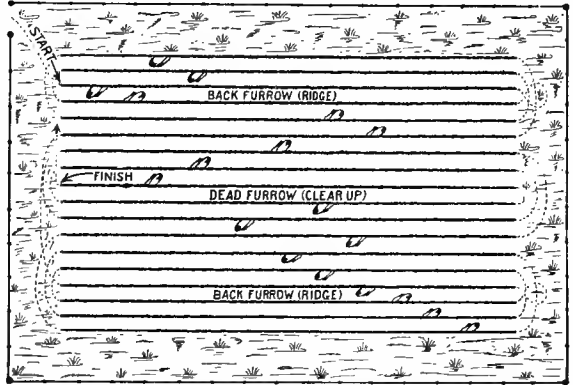
Illust. 40. Plowing the center of the field out in lands is the most common method. This shows one of the best plans for plowing out the lands in order to reduce idle running at the ends and eliminate about half the dead furrows. Plow symbols show direction dirt is thrown.
