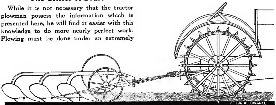
Illust. 32. Of the dotted lines the straight line shows the true line of draft with respect to the height of the plow hitch and the tractor drawbar. The other dotted lines show high and low hitch. The bent lines will straighten under load and the working of the plow will be affected accordingly.
