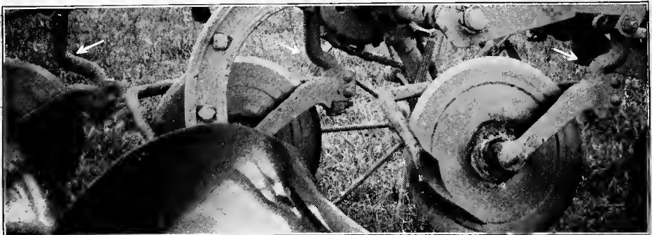
Illust. 5. When the coulters are properly set, they will line up as shown above. Notice the angle at which the offsets in the couler shanks set—front one toward the rear and the second and third toward the front.
