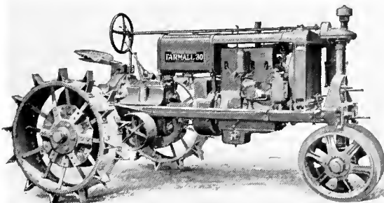
Illust. 54. Farmall 30, the 3-plow size of the famous Farmall.
