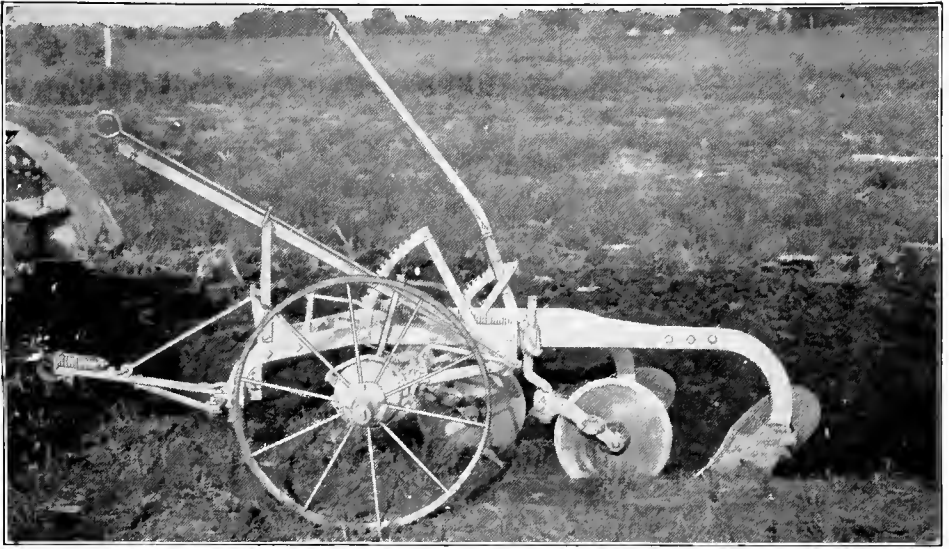
Illust. 1. This plow is set for one hundred per cent perfect work. Both bottoms will turn furrows exactly the same width and depth. The hitch is at the correct angle, neither too high nor too low, and a minimum amount of power will be required to pull the plow. To obtain this result the adjustments noted in the following pages are required.
