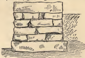
ILLUSTRATION 29.—Bond Rubble.
