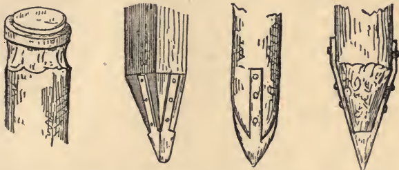
ILLUSTRATION 7.—Wrought or Cast-iron Shoes to Piles.
