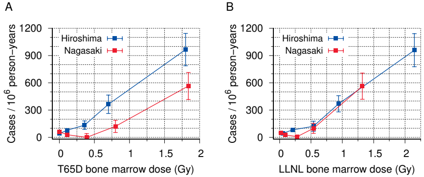
Figure 11.4 Leukemia rates vs. T65D bone marrow dose estimates (A, Rossi and Mays [229]) and preliminary revised ones (B, Loewe and Mendelsohn [92]) prepared by the Lawrence Livermore National Laboratory (LLNL). The dose values comprise estimates for both \gamma -rays and neutrons. Error bars represent standard deviations.
