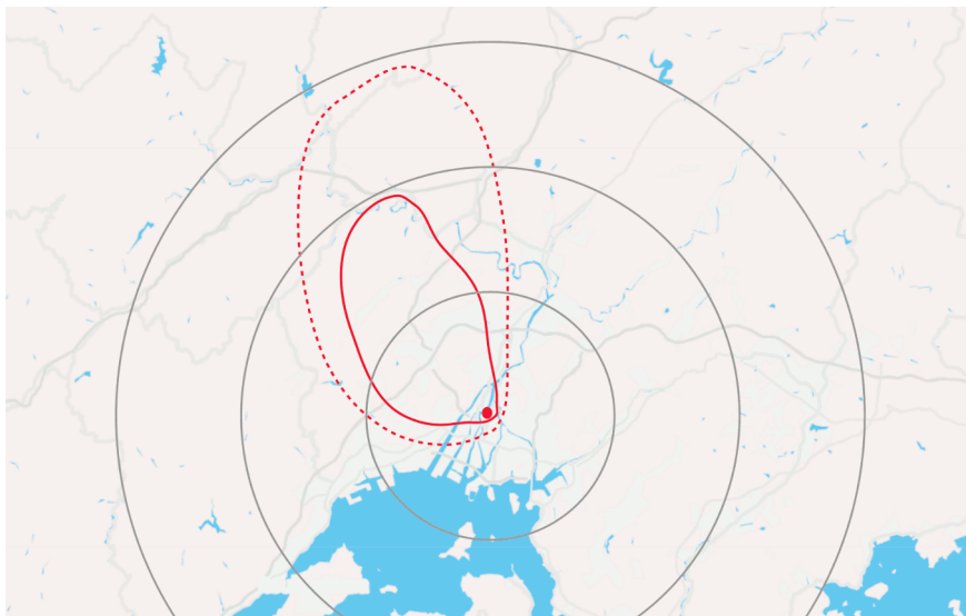
Figure 3.1 Area affected by black rain in and near Hiroshima. The areas of heavy and light black rainfall extend in NWN direction from the hypocenter (red dot) and are indicated by solid and dashed red outlines, respectively. Concentric rings indicate distances of 10, 20, and 30 km from the hypocenter. Drawn after a similar map in [57]. The studies cited in this chapter mostly used soil samples from within the heavy black rain area.
