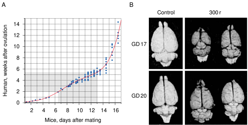
Figure 12.1 Time correlation of mouse and human embryonic development, and time-dependent effect of prenatal irradiation on brain growth in rats. A: Data points replotted from Otis and Brent [232]. Each point represents a specific organ development milestone. Highlighted in gray is the phase most susceptible to radiation-induced malformations in the mouse [231] and its equivalent in humans, estimated from the fit polynomial (red). B: Reduced brain size in rats after irradiation with an X-ray dose of 300 r (approximately 3 Gy) on gestational days (GD) 17 and 20, respectively. Adapted from Hicks [233].
