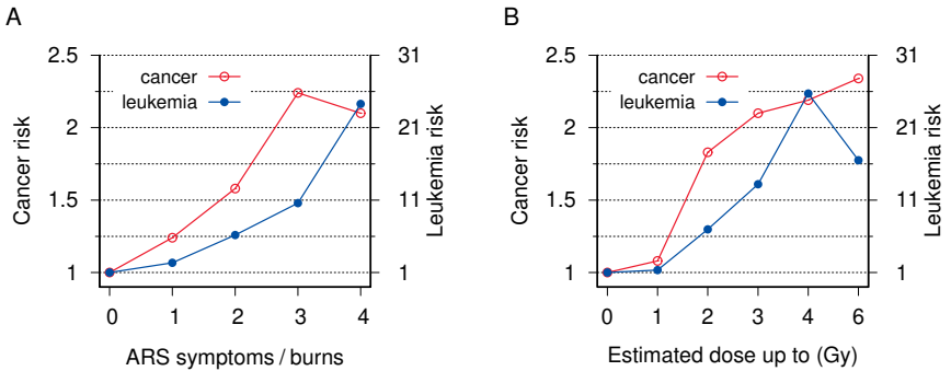
Figure 12.5 Risk of death due to cancer and leukemia vs. number of clinical symptoms (A) and radiation dose estimates (B). Symptoms comprise three proper signs of ARS (epilation, bleeding, and oropharyngeal lesions), and burns are counted here as a fourth symptom. Risks are relative to zero symptoms (A) or zero Gy (B). Data from [168]; in both A and B, only subjects with unambiguous information for all three ARS symptoms and for burns were included (these account for > 90% of the total).
